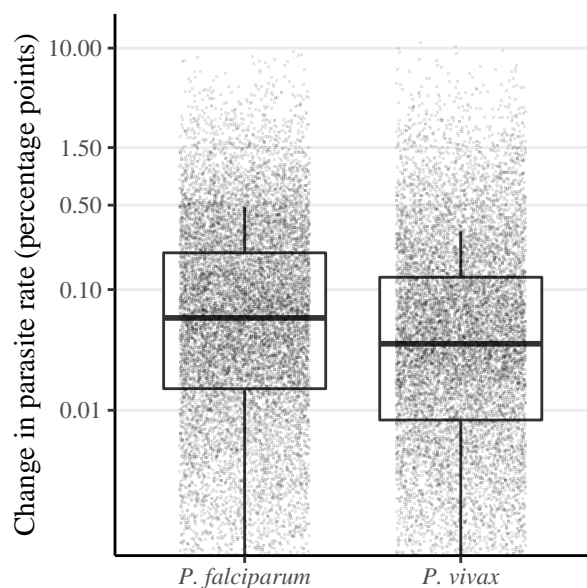
Figure 3: Increases in parasite rate.
