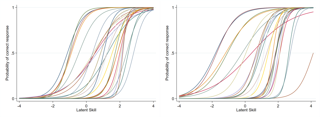
(a) Matrix Reasoning Test
