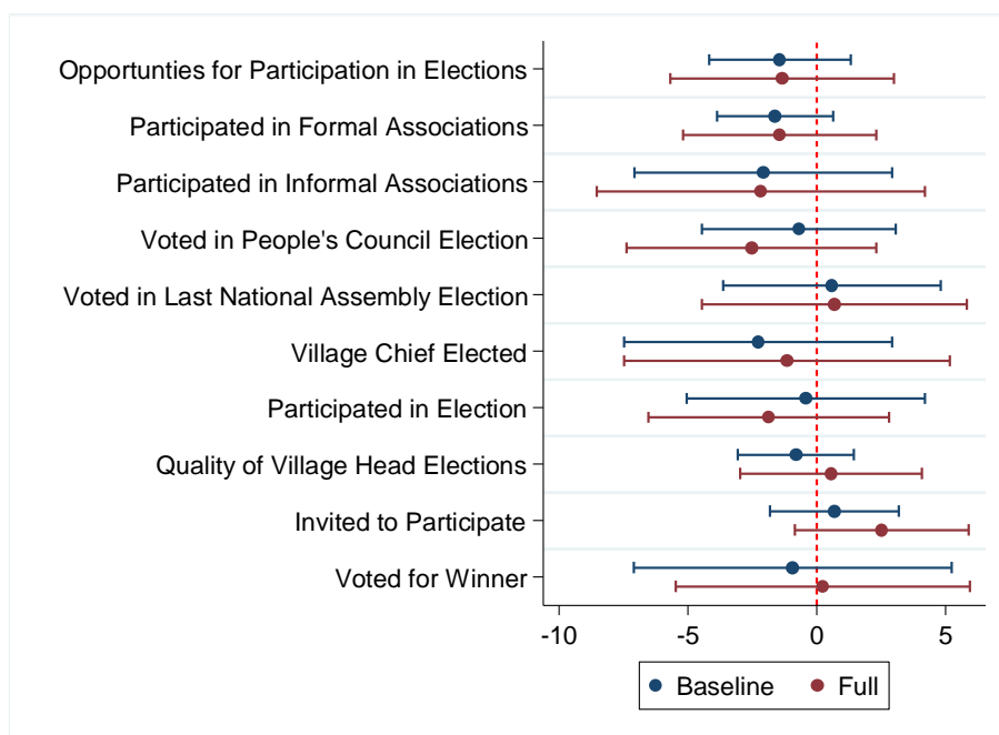
Figure 6: Relationship between participation and death cases
