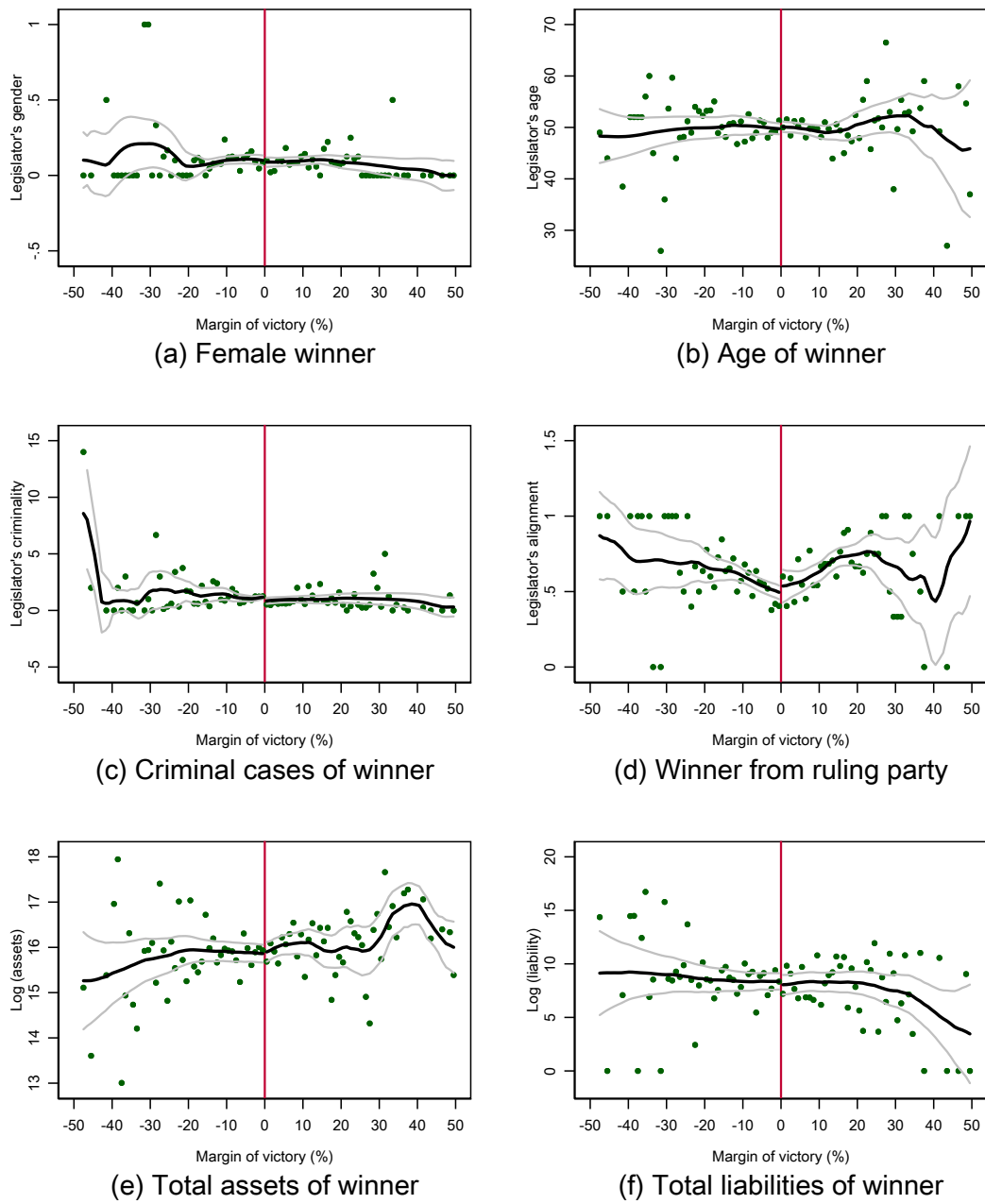
Figure 3: Continuity checks of candidate characteristics
