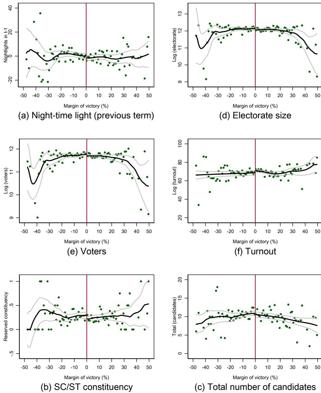
Figure 2: Continuity checks of constituency-level covariates
