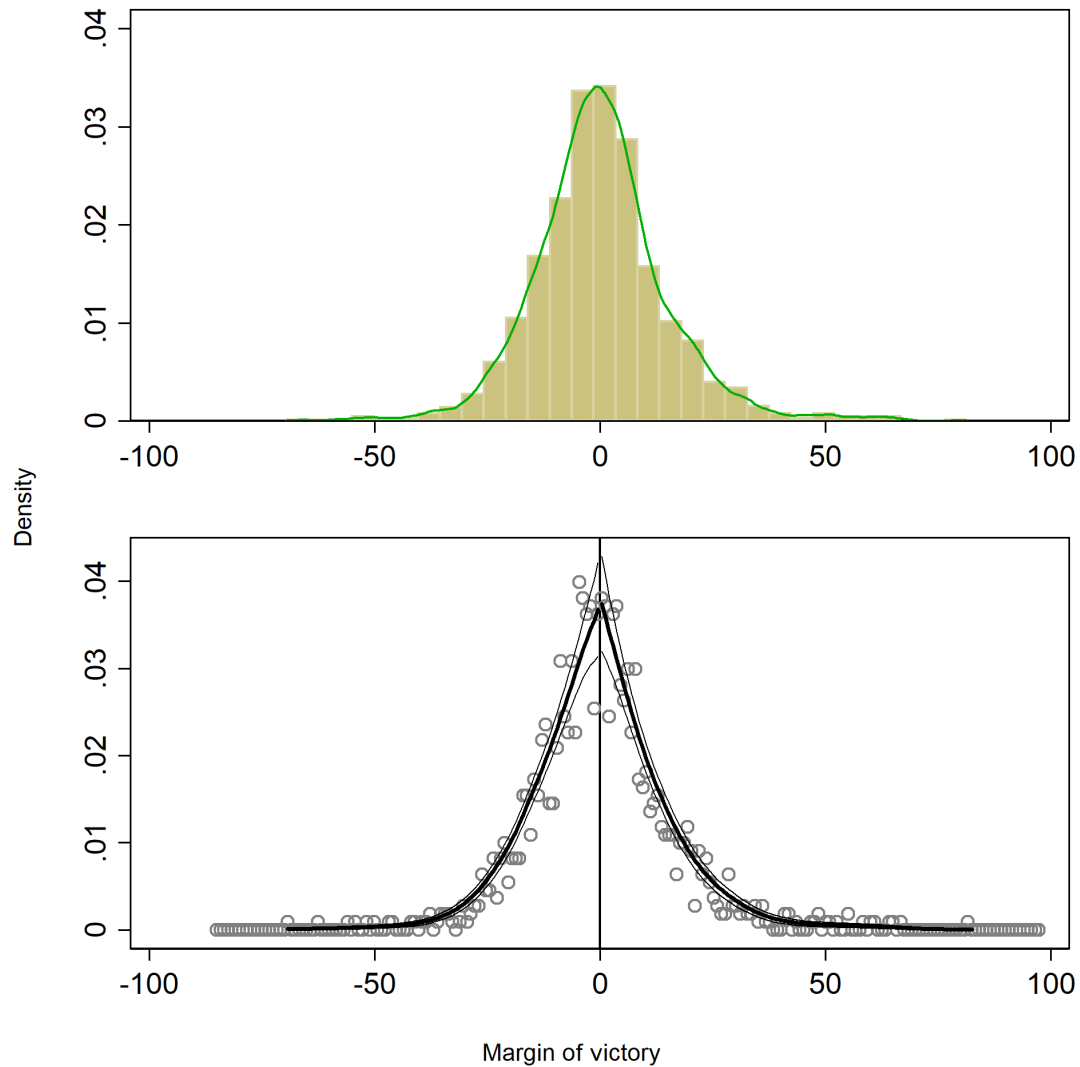
Figure 1: Density test of the forcing variable
