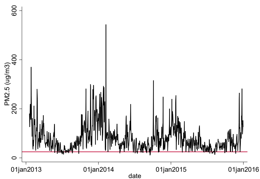
Figure A2 Daily mean PM2.5 ( \mu\text{g}/\text{m}^3 ) in Wuhan city, 2013-2015
