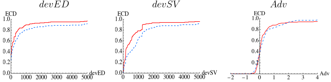
Figure 3: Empirical cumulative distribution of devED , devSV , and Adv
