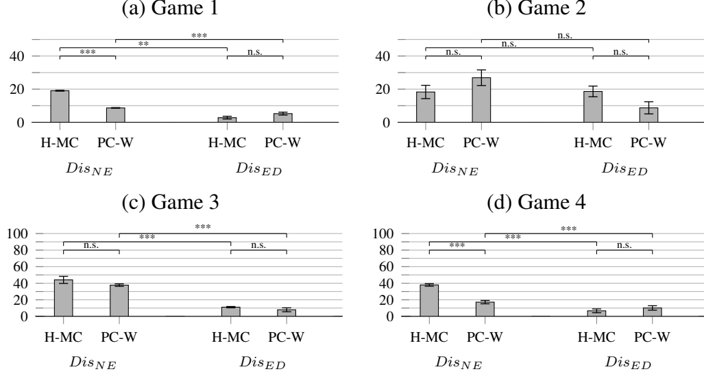
Figure 6: Mean of the distances of the realized payoff vectors from the subgame perfect Nash equilibrium and the equal division
