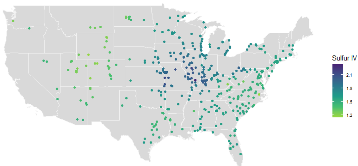
(b) Weighted average of median sulfur content of available coal by inverse distance for all coal-fired power plants.
