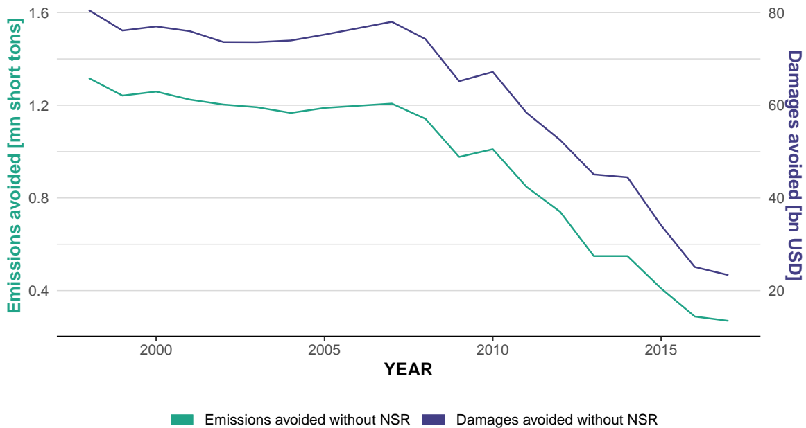
Figure 5: Total SO x emissions and damage effects from NSR
