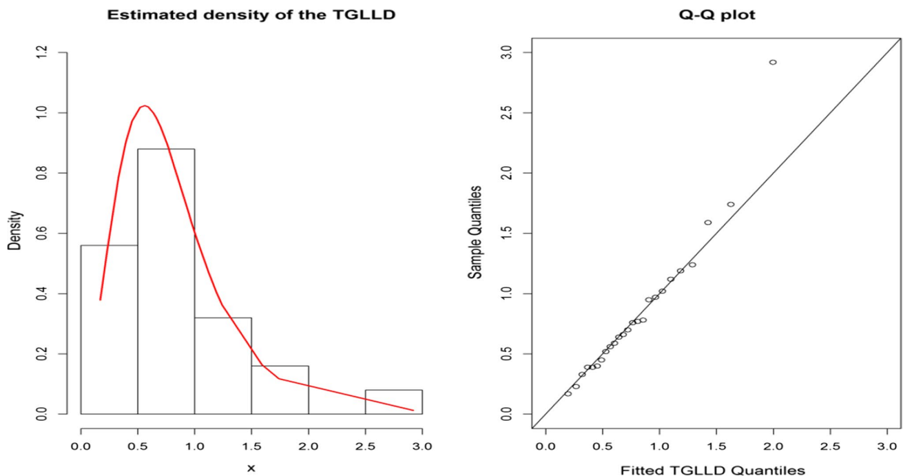
Fig. 1 Density plot and Q–Q plot of the fitted type-II generalized log-logistic distribution for the runoff amounts data
