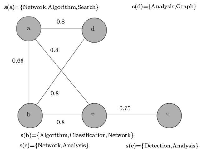
Fig. 4 The relationship between experts
