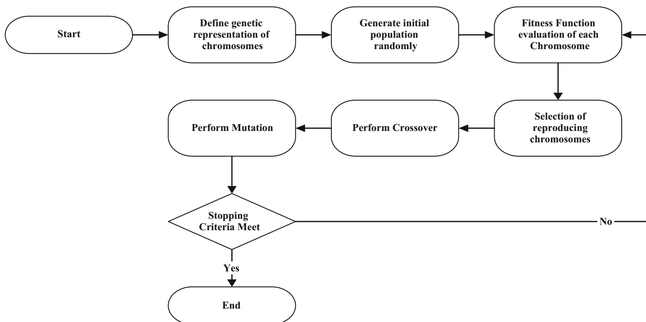
Fig. 6 Procedure of Genetic Algorithm
