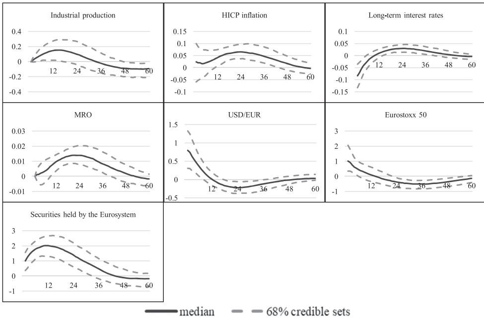
Figure 16. Robustness check V: using MRO rate as a proxy for standard monetary policy actions.
