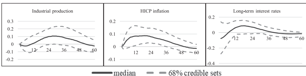
Figure 3. BSVAR-BE results for Latvia.
