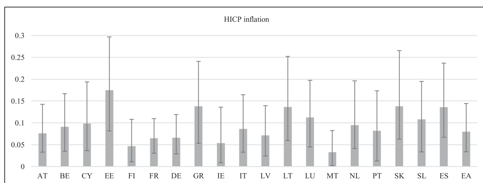
Figure 11. MCS-BGVAR-SV country-level results: inflation.
