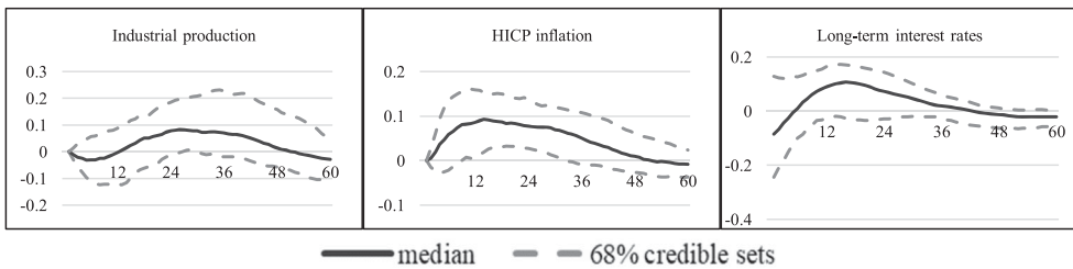
Figure 17. Robustness check VI: identifying LV-specific shocks.
