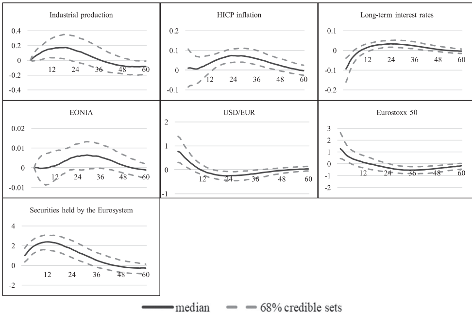
Figure 1. BSVAR-BE results for the euro area.
