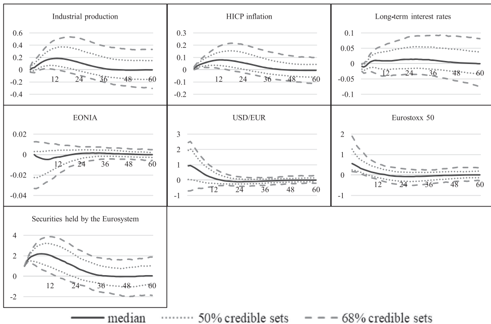
Figure 2. MCS-BGVAR-SV results for the euro area.
