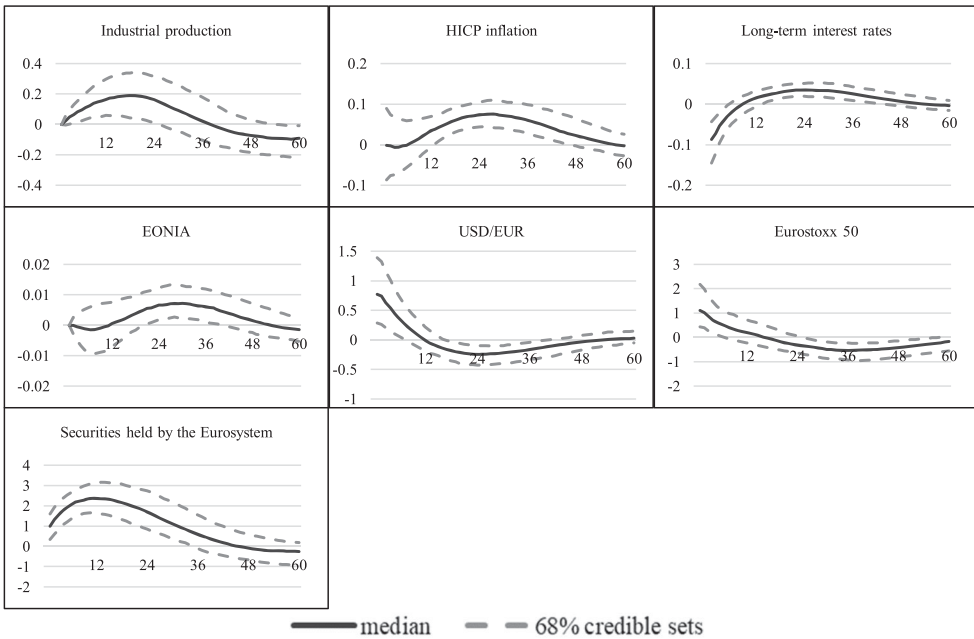
Figure 15. Robustness check IV: controlling for the central bank information shocks.
