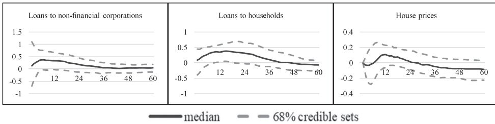
Figure 6. BSVAR-BE results: the financial channel.
