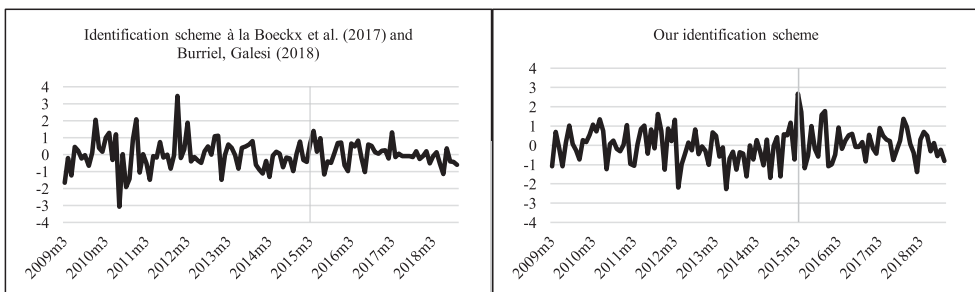
Figure 13. Robustness check II: comparison of the shock time series.
