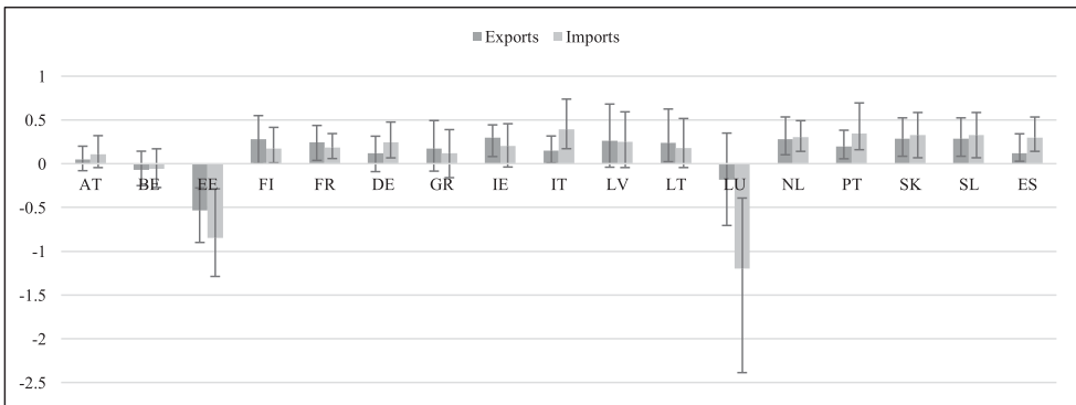
Figure A3. MCS-BGVAR-SV country-level results: trade with the extra-euro area.
