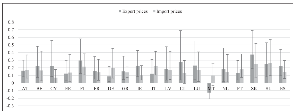
Figure A4. MCS-BGVAR-SV country-level results: trade prices with the euro area.
