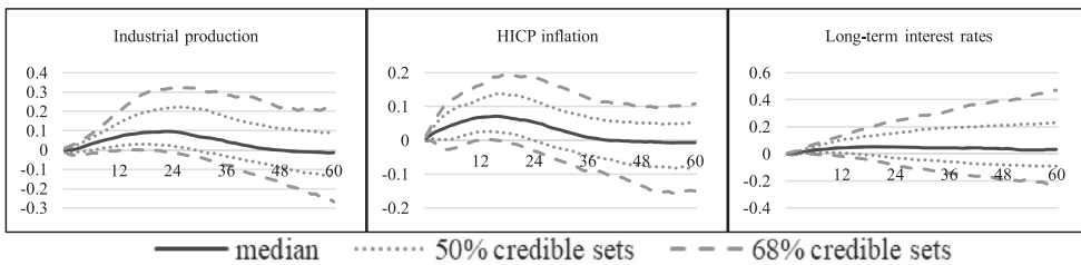
Figure 4. MCS-BGVAR-SV results for Latvia (total impact).
