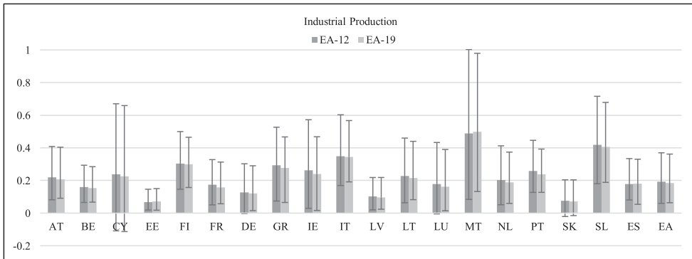
Figure A6. MCS-BGVAR-SV country-level results: output.
