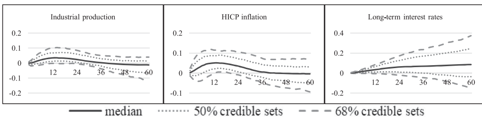
Figure 5. MCS-BGVAR-SV results for Latvia (direct impact).
