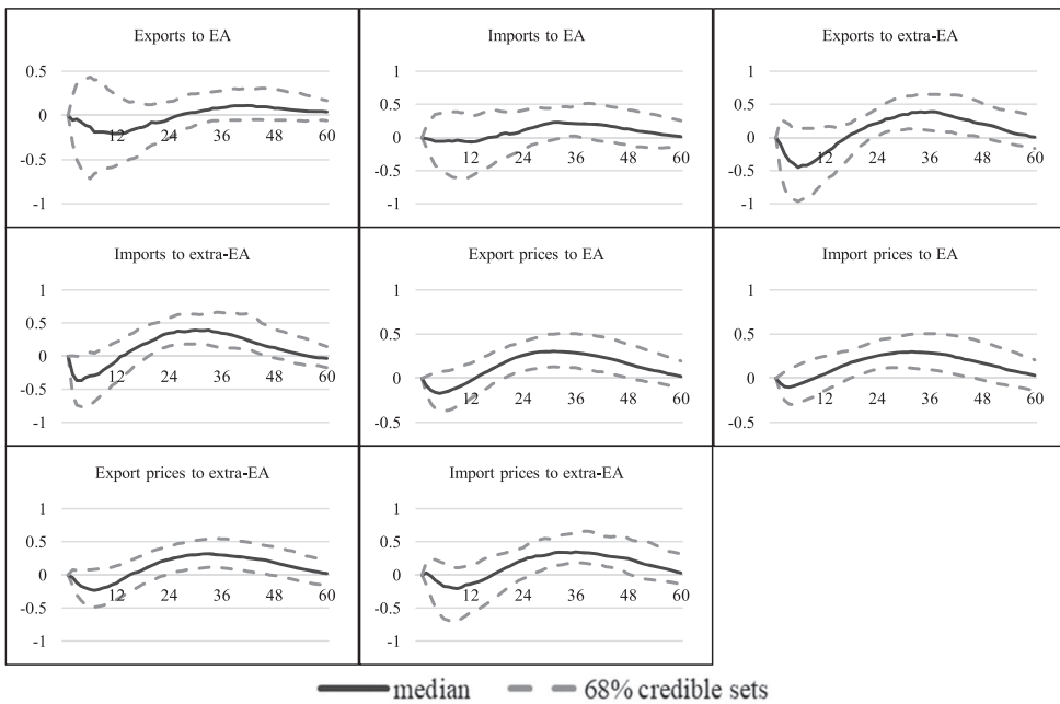
Figure 8. BSVAR-BE results: the trade channel.
