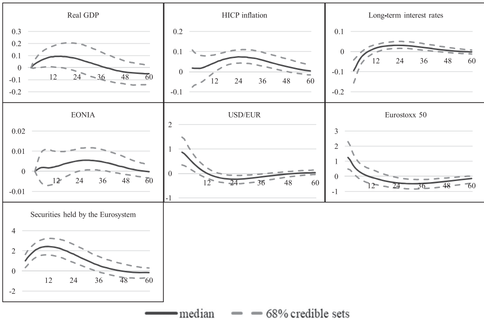
Figure 12. Robustness check I: real GDP as measure of output.
