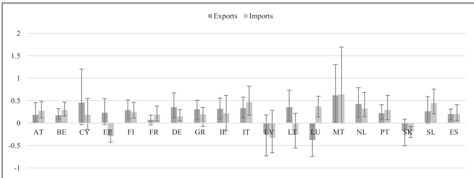
Figure A2. MCS-BGVAR-SV country-level results: trade with the euro area.
