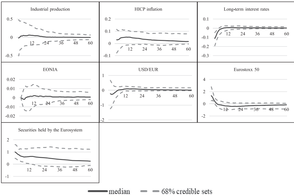
Figure 14. Robustness check III: using a pre-APP data sample (January 2009 – August 2014).
