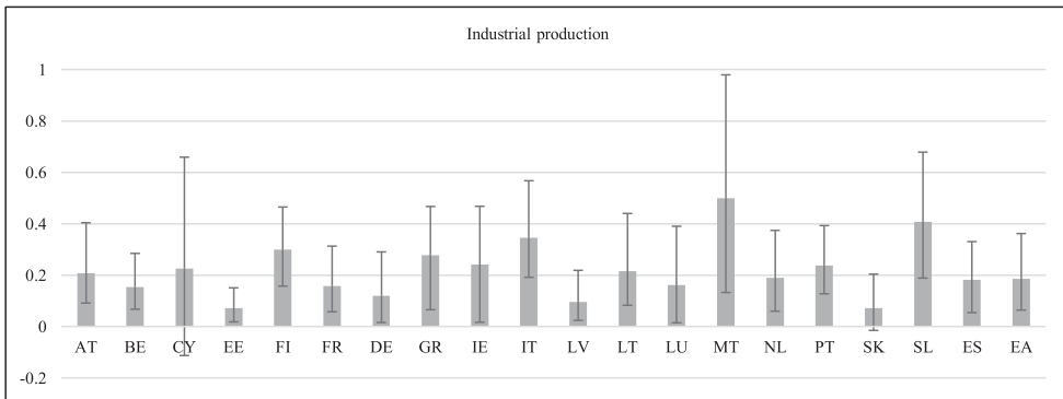
Figure 9. MCS-BGVAR-SV country-level results: output. 11
