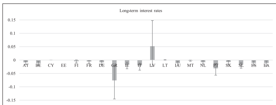
Figure 10. MCS-BGVAR-SV country-level results: sovereign yields.
