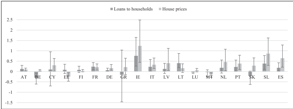
Figure A1. MCS-BGVAR-SV country-level results: the financial channel.
