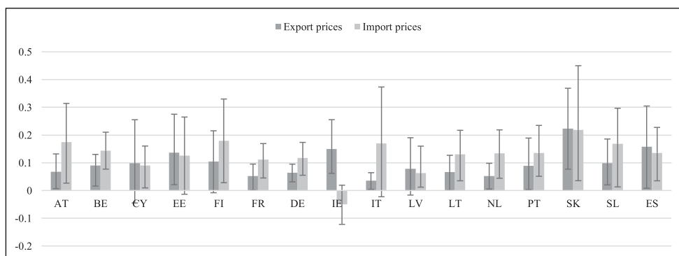
Figure A5. MCS-BGVAR-SV country-level results: trade prices with the extra-euro area.
