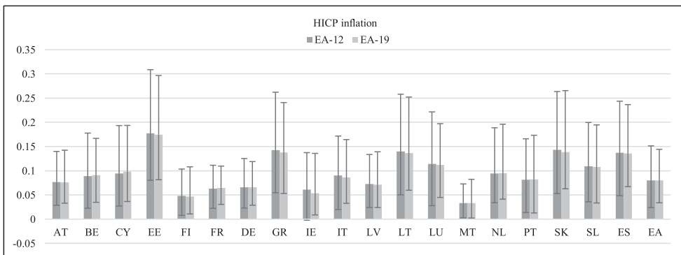
Figure A8. MCS-BGVAR-SV country-level results: inflation.
