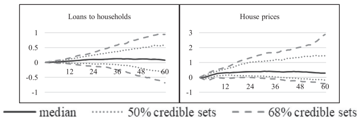
Figure 7. MCS-BGVAR-SV results: the financial channel.
