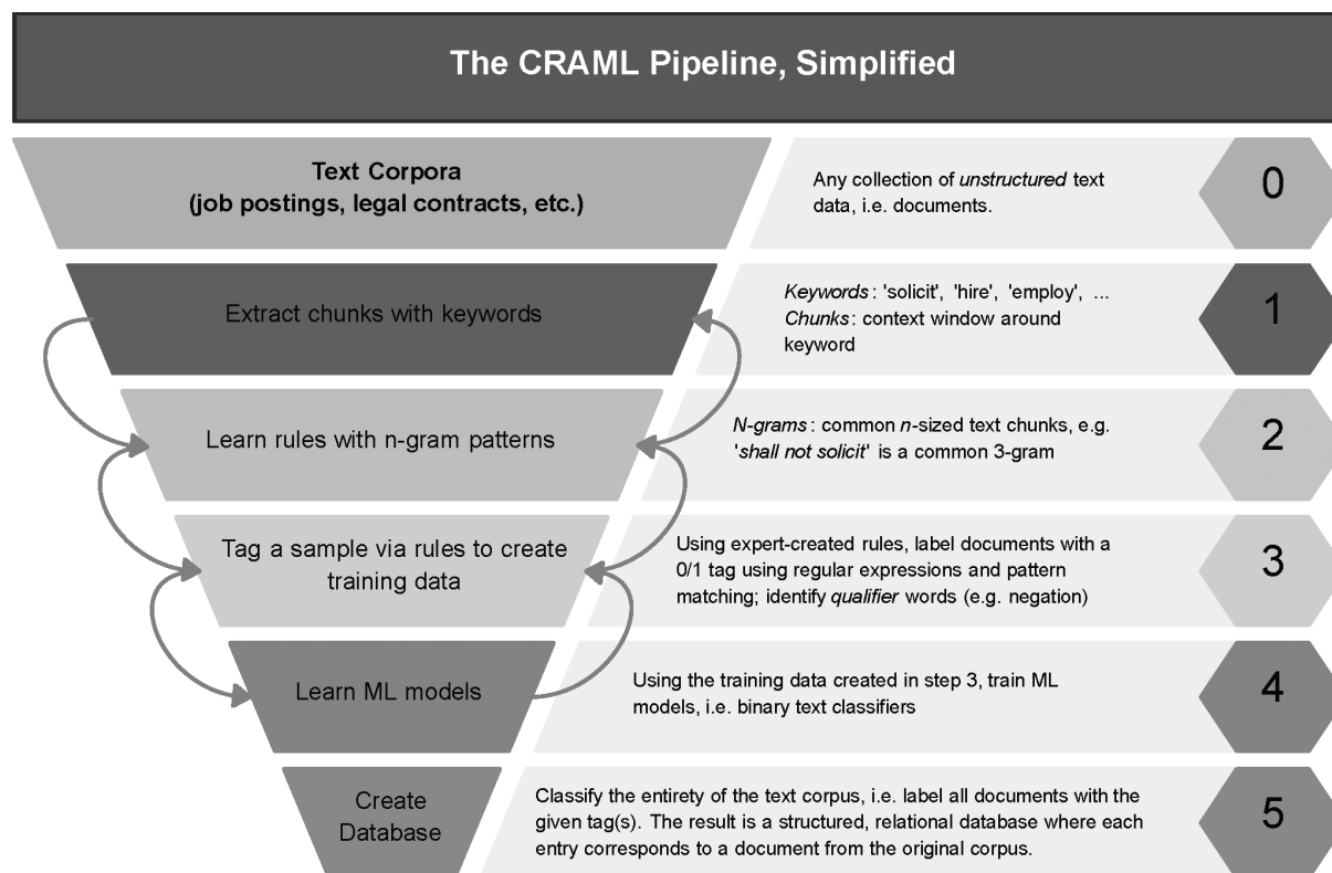
Figure 2: A Bird’s Eye View of the CRAML Process
