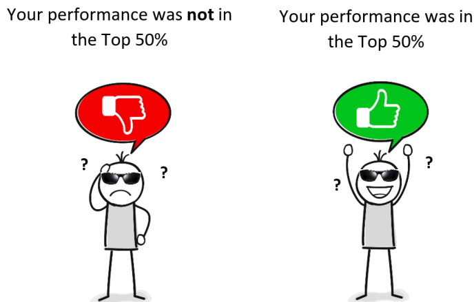
Figure 4: Signal realization
