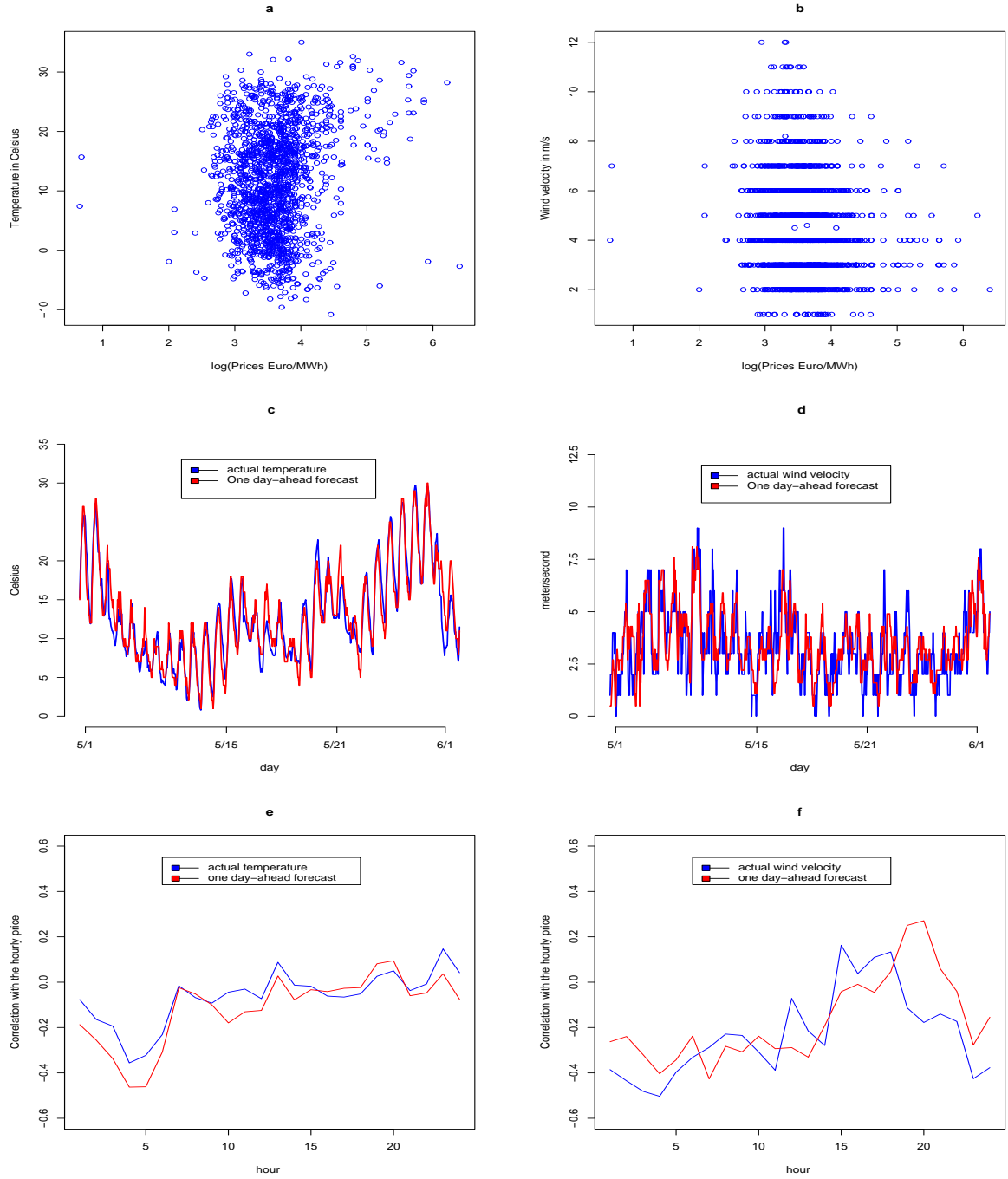
Figure 1: Scatter plots for temperature from Ulm and wind velocity from Holz- dorf ( hour 12 ) with the logarithm of the hourly price series (hour 12) (a,b), one day-ahead forecasts for temperature from Ulm and for wind velocity from Holz- dorf (c,d), for 7 a.m. 1/05/2005 until 6 a.m. 1/06/2005, Correlation of measured temperature from Ulm and wind velocity from Holzdorf as well as its one day- ahead forecasts with the hourly price for 7 a.m. 1/05/2005 until 6 a.m. 1/06/2005 (e,f).
