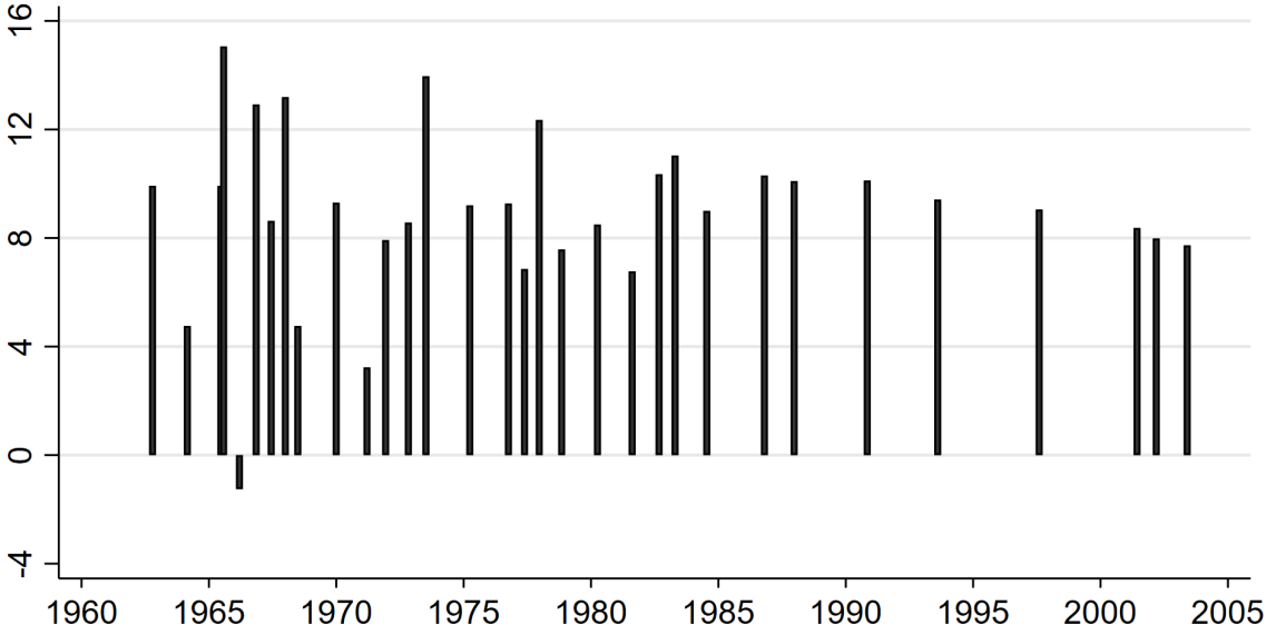
Figure 1: The Flesch-Kincaid Grading Level of Tax Bills
