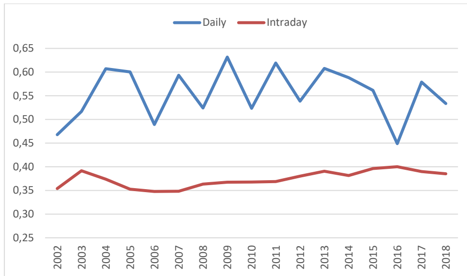
Figure 2: Dynamics of the Hurst exponent during 2002-2018: daily and intraday data
