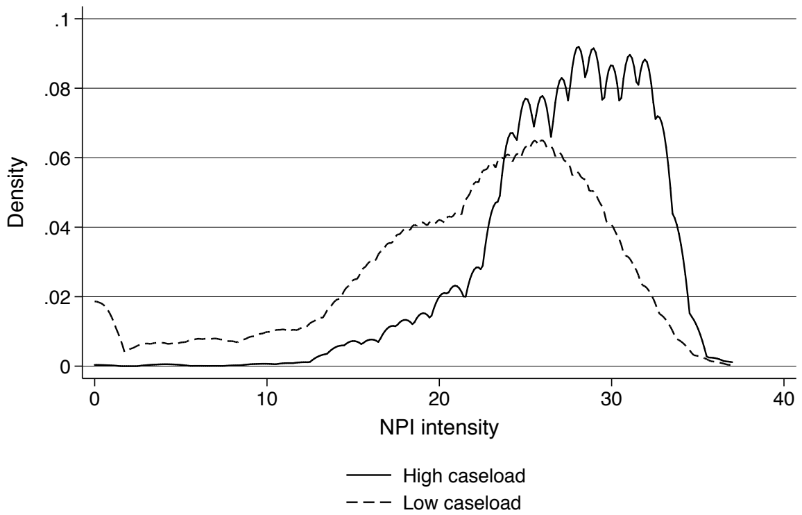
Figure B.5: Distribution of NPI intensity
