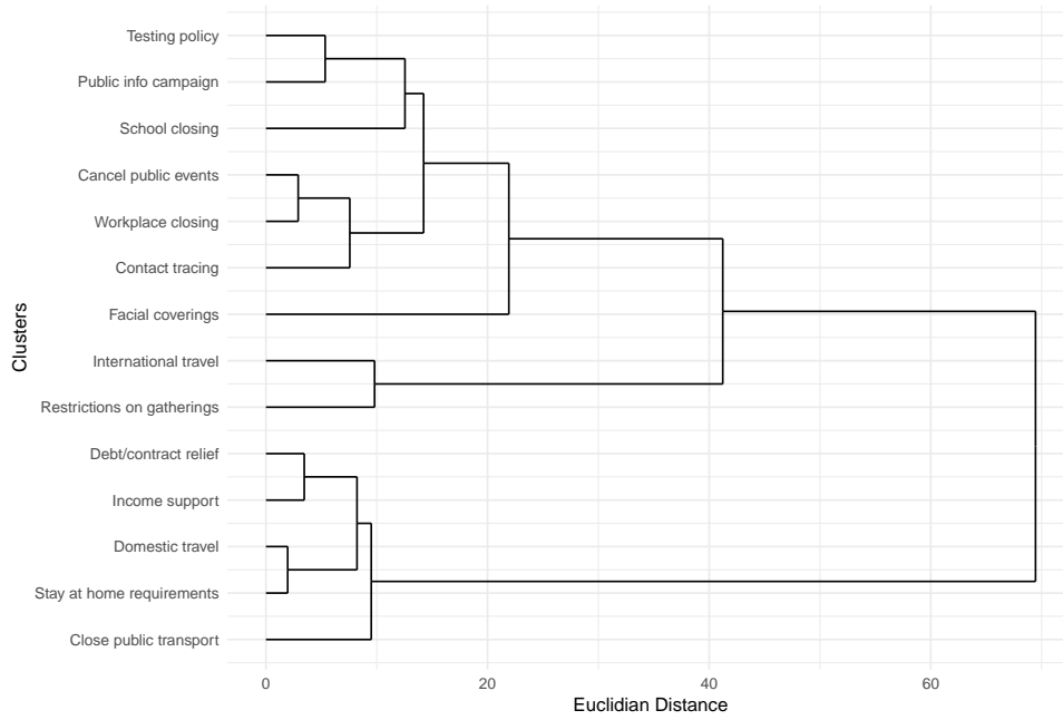
Figure B.4: Hierarchical temporal clustering of NPIs
