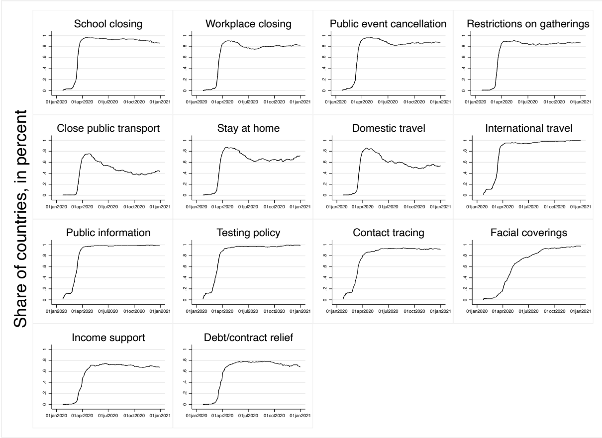
Figure 1: NPI rate of implementation in 2020
