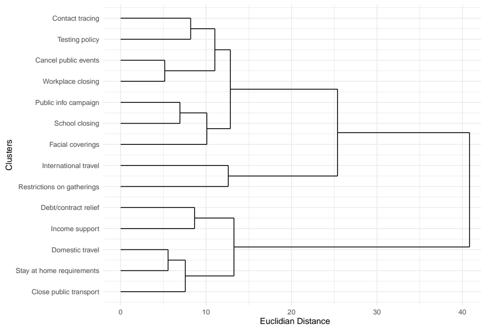
Figure B.3: Hierarchical sectional clustering of NPIs
