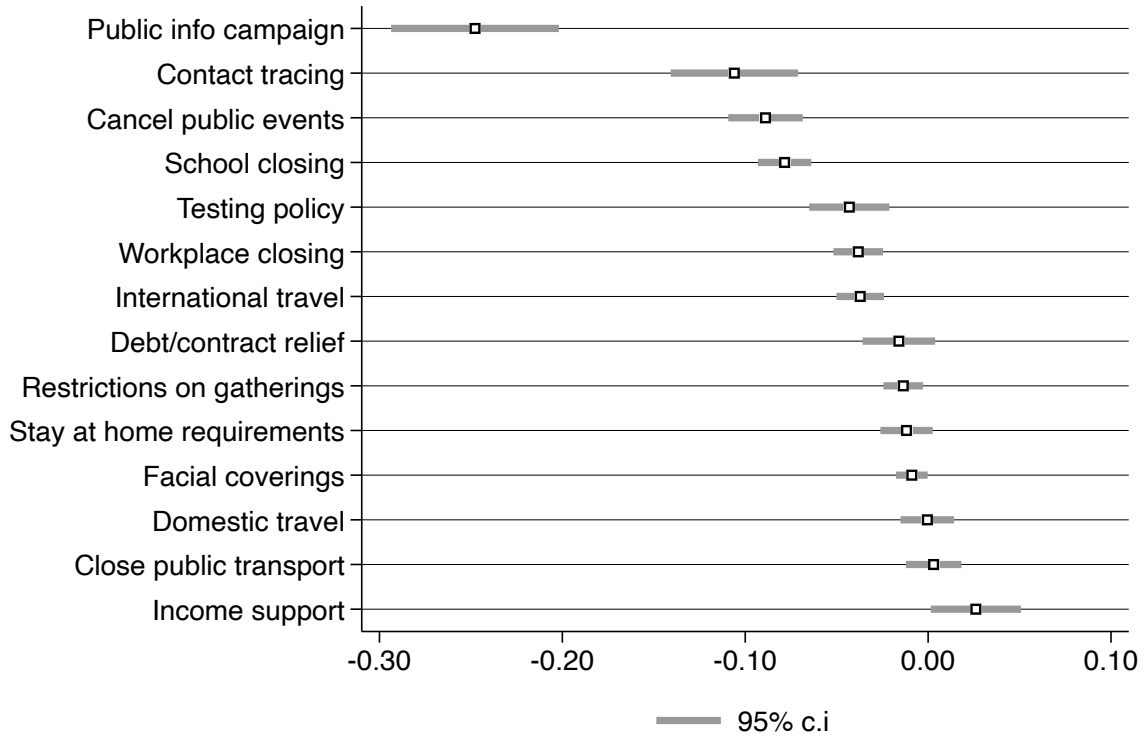
Figure 2: Ranking of NPIs
