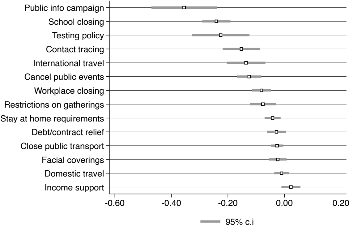
Figure 3: Ranking of dummy NPIs
