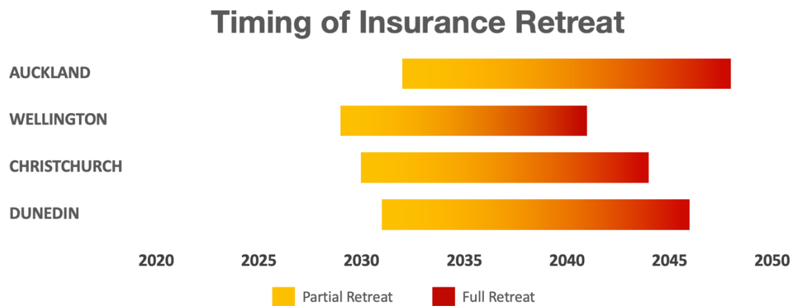
Figure 5: Timing of modelled insurance retreat for properties in the 1% AEP (1:100 ARI) coastal inundation zones per port-city. Note this analysis uses Sea Level Rise from RCP 4.5 (MfE, 2017), Gumbel distributions using data to 2019. Authors' own graphic.
