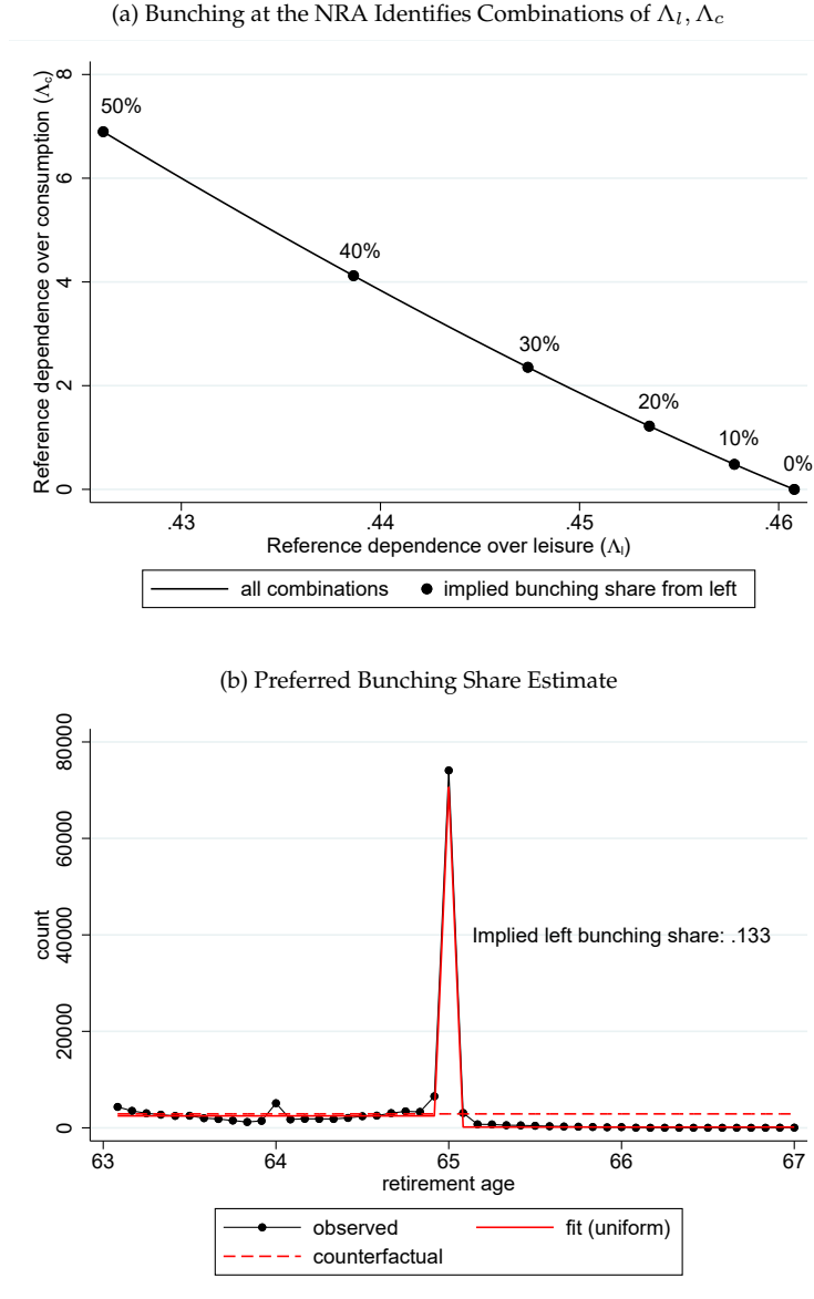
FIGURE A5: TWO-DIMENSIONAL REFERENCE DEPENDENCE
