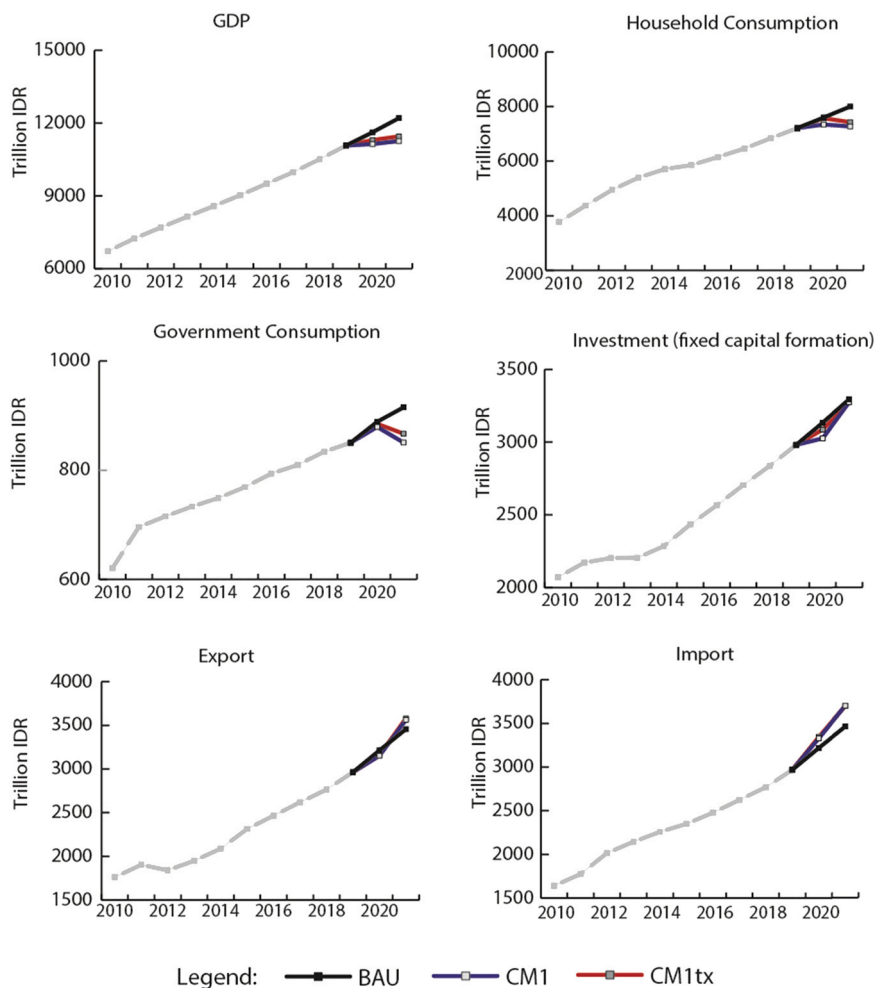
Fig. 3. Results of the simulation for macroeconomic indicators under each scenario.
