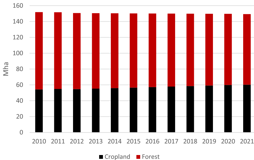
Fig. 2. Available land for cropland and forestland in Indonesia in 2010–2021. This cropland can be cultivated for agricultural activities (in this study, for food crops, plantations, wood, and livestock). Source: Derived from (Boer et al., 2016).
