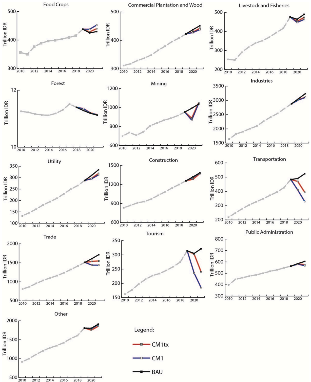
Fig. 4. Results of the simulation for sectoral GDP under each scenario Notes: Food Crops include all carbohydrate sources (e.g., paddy, corn, cassava) and horticulture (e.g., vegetables and fruits). The detailed sector classification and grouping can be found in the Appendix (Table 2B).
