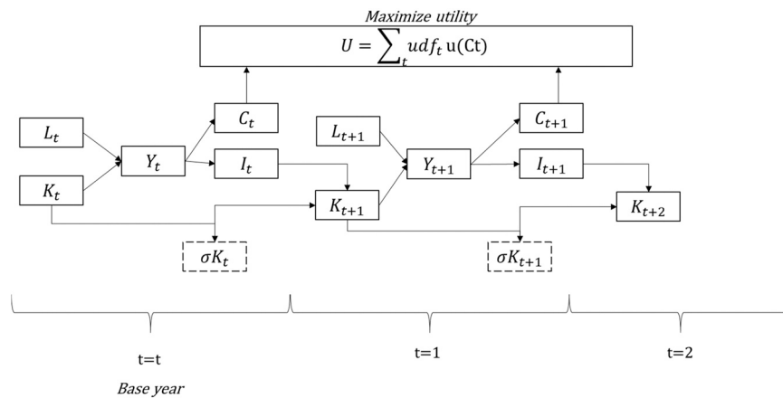
Fig. A1. Illustration of the recursive dynamic process in calculating the capital stock and maximizing the utility. Notes: U : Social Utility; C : Final Consumption; I : Investment (saving); K : Capital stock; Y : Production; L : Labour; udf : Utility discount factor; \delta : Depreciation rate; f (·): Production function; u (·): Utility function. Source: (Malahayati and Masui, 2021).
