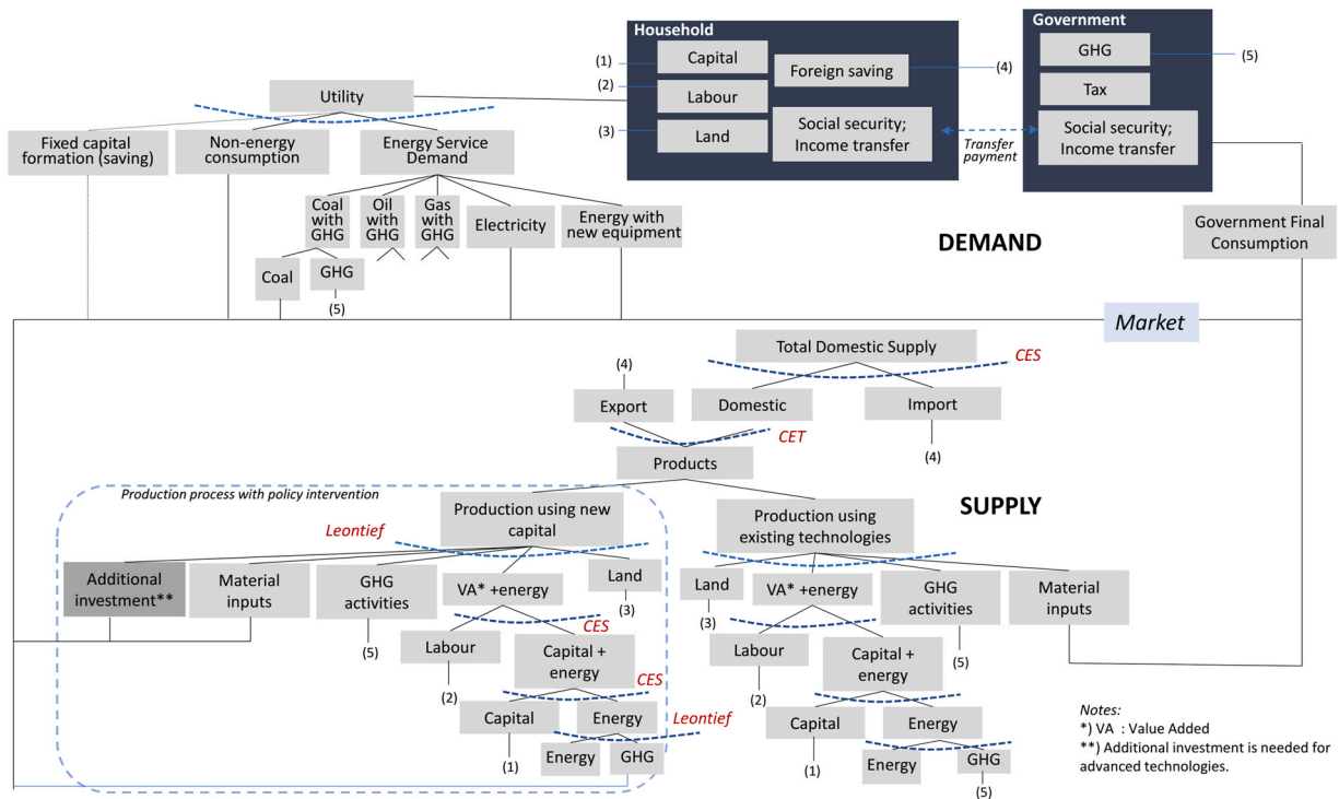
Fig. 1. Model structure of the study. Notes: CES: constant elasticity of substitution, CET: constant elasticity of transformation (substitution elasticity relation). CES is often used to describe the relation between price and demanded quantity (e.g. a lower price means higher demand). In contrast, CET is used to describe price and supplied volume relation (e.g., higher export price, higher export). Source: Malahayati, 2019.
