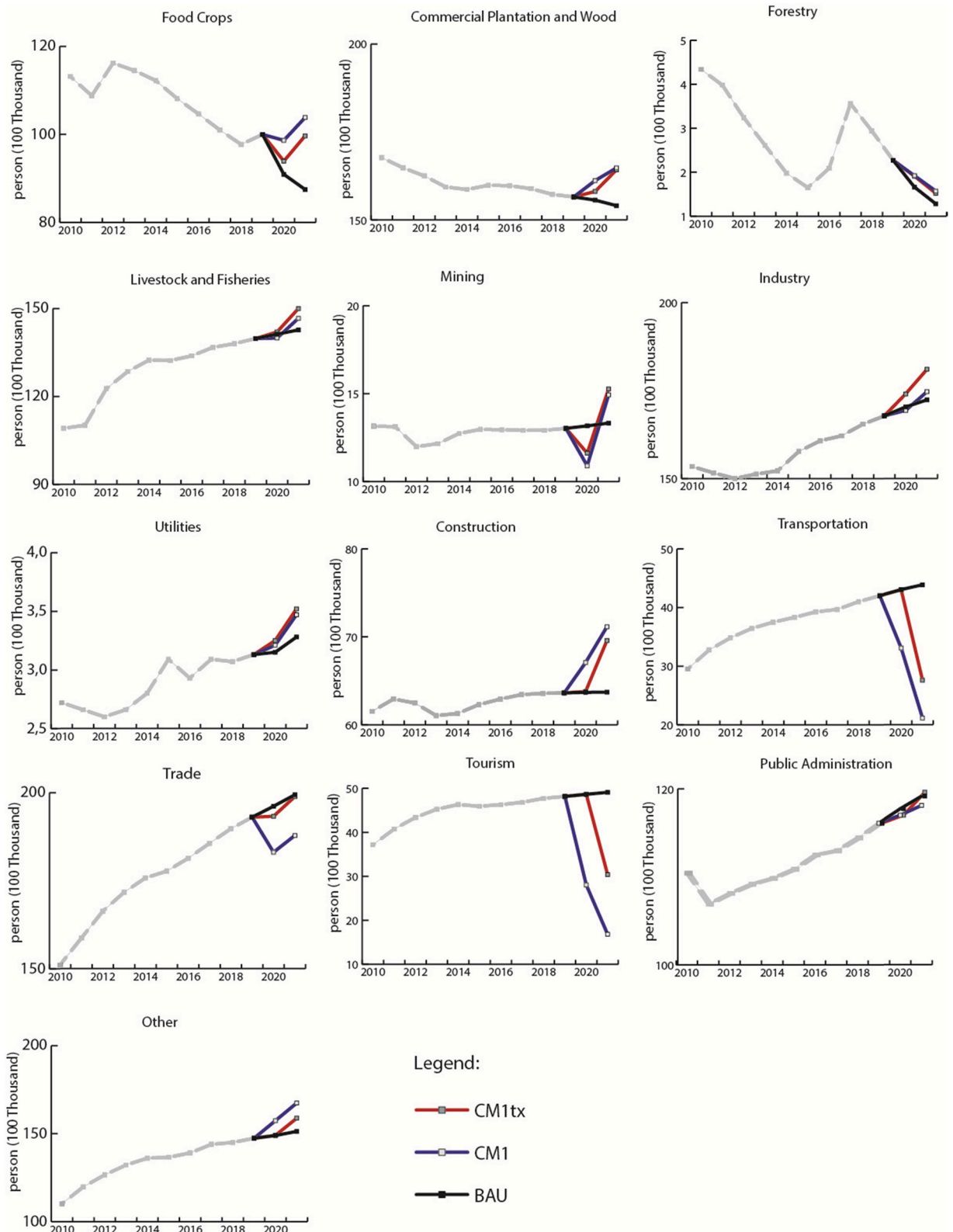
Fig. 5. Results of the simulation result for labour under each scenario.
