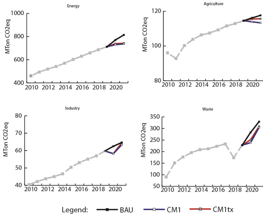
Fig. 7. Sectoral GHG emission under each scenario Notes: 1) The emissions from land-based sectors are summarised in 'agriculture' (food crops, plantations, woods, livestock, and forest). 2) The emissions from agriculture only counting the emissions from agricultural activity (not include emissions from land use change).
