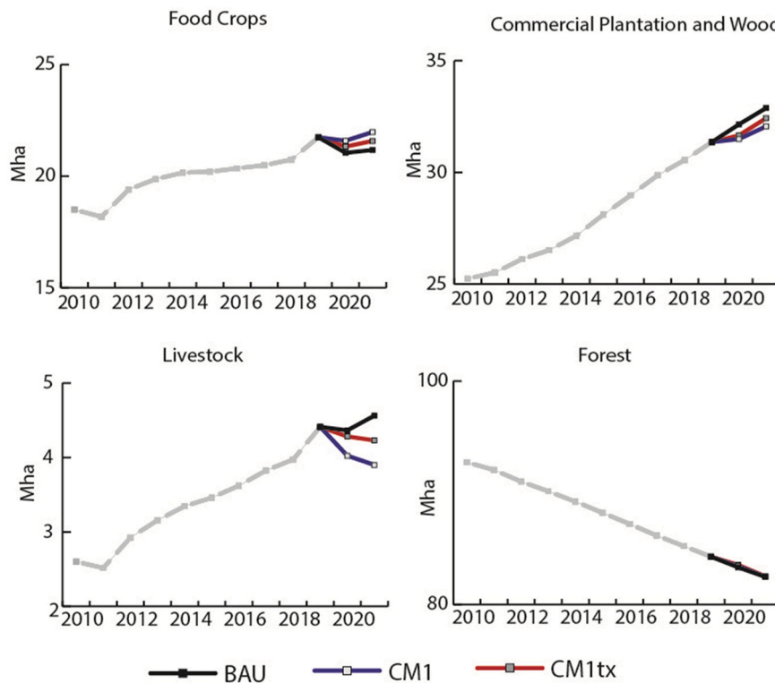
Fig. 6. Result of the simulation on demand for land under each scenario.
