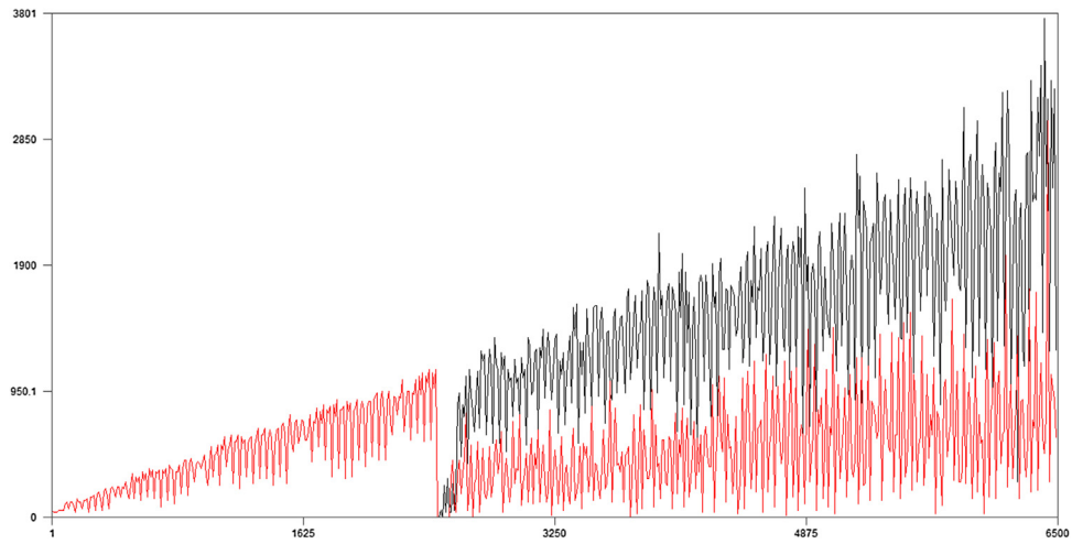
Fig. 3. Average Level of Inventories in test ii (black) and test iii (red) - Pessimism Shocks.
