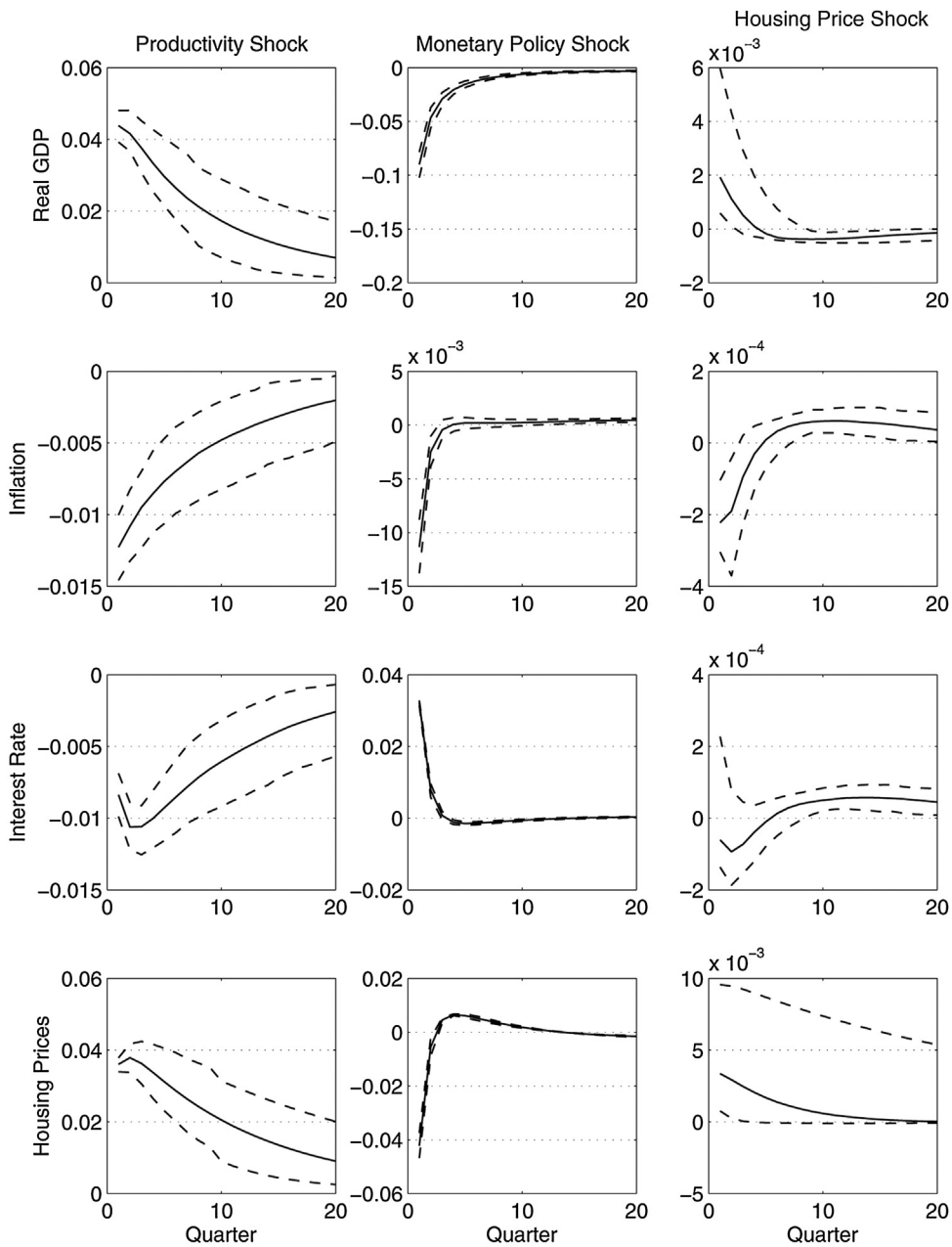
Fig. 1. Theoretical IRF. Note: The solid line depicts the median response, while the dashed lines represent the 68% highest-posterior density interval.
