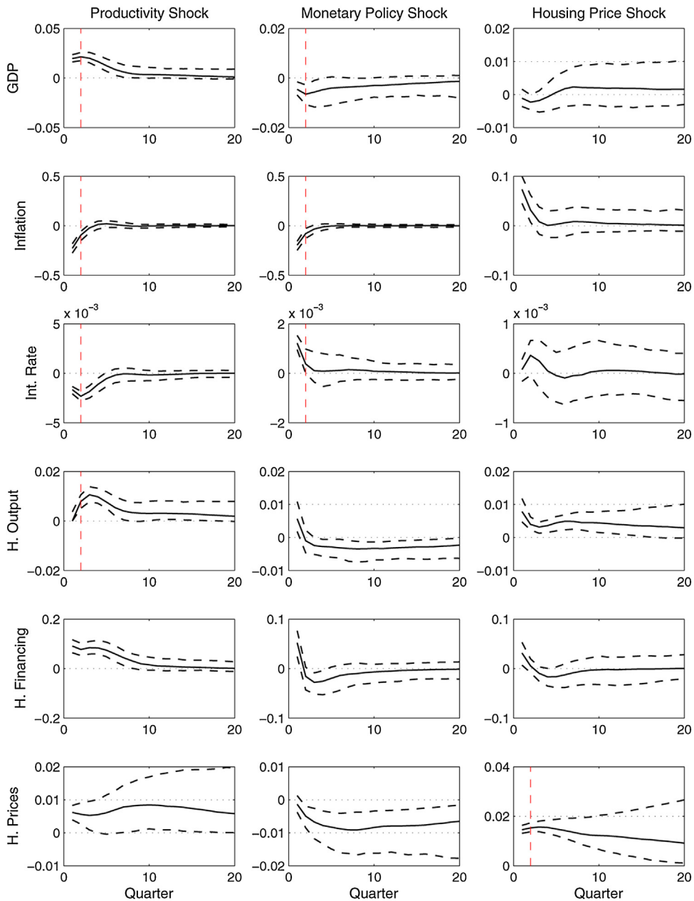
Fig. 5. Empirical IRF: lower restriction k = 2 quarters. Note: The solid line depicts the median response, while the dashed lines represent the 68% confidence interval. The vertical line represents the sign restriction horizon k = 2 quarters.
