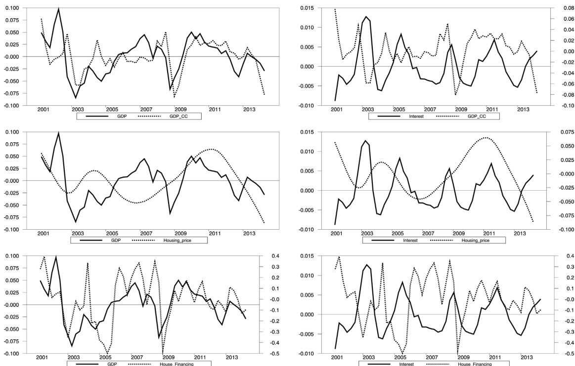
Fig. 2. Housing market series. Note: Housing market variables and aggregate real GDP are in logs and HP filtered ( \lambda = 1600 ). The nominal interest rate is HP filtered only.
