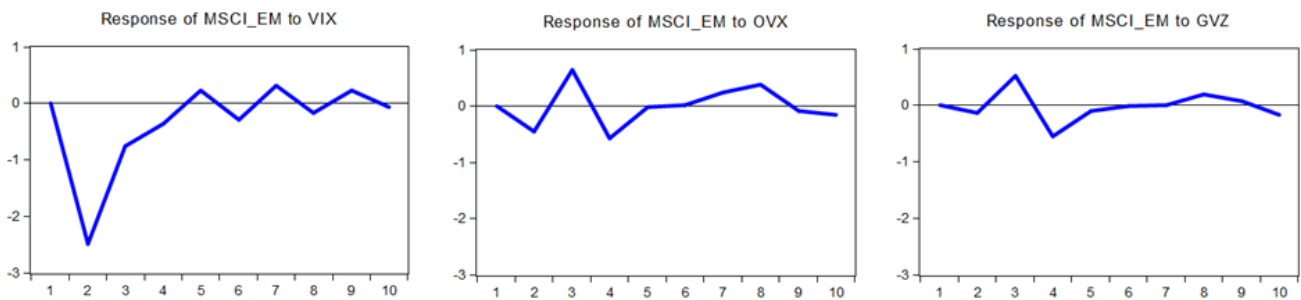
Graph 3: Impulse-Response analysis
