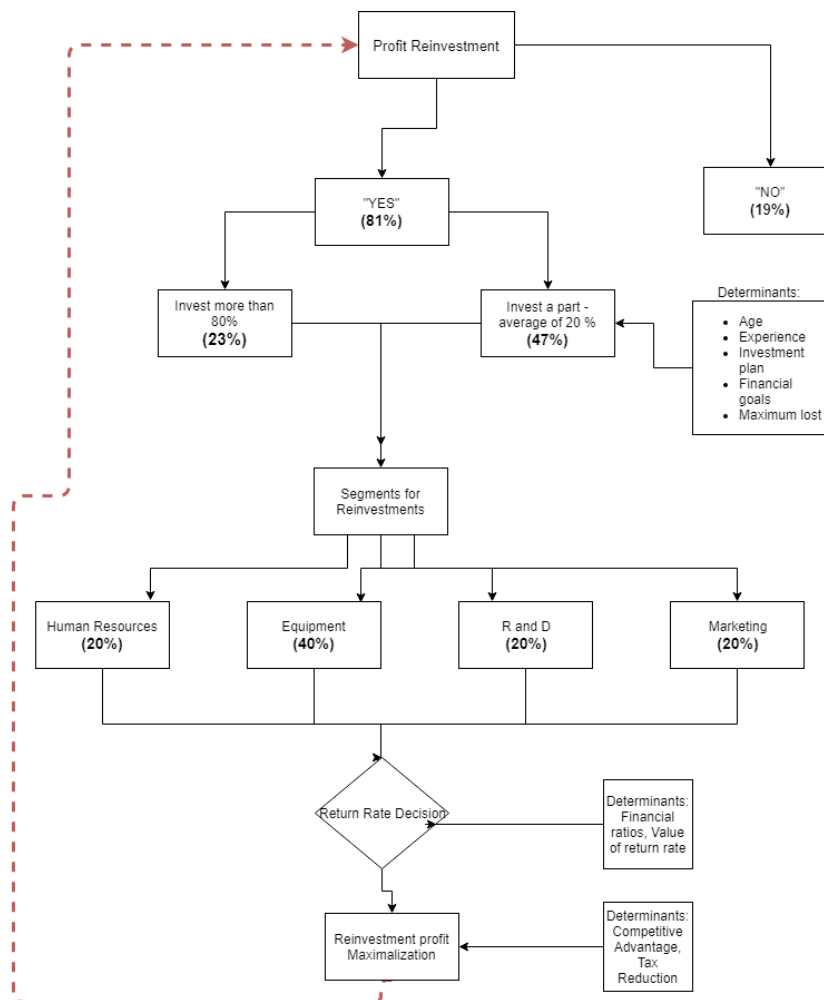
Figure 2: Decision-making tree
