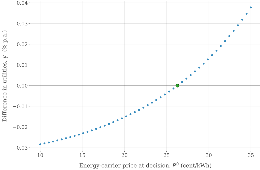
FIGURE 4. The utility difference \gamma (Equation 7) as a function of gas price at the moment of decision P^0 . The trigger price P^* is indicated in green.
