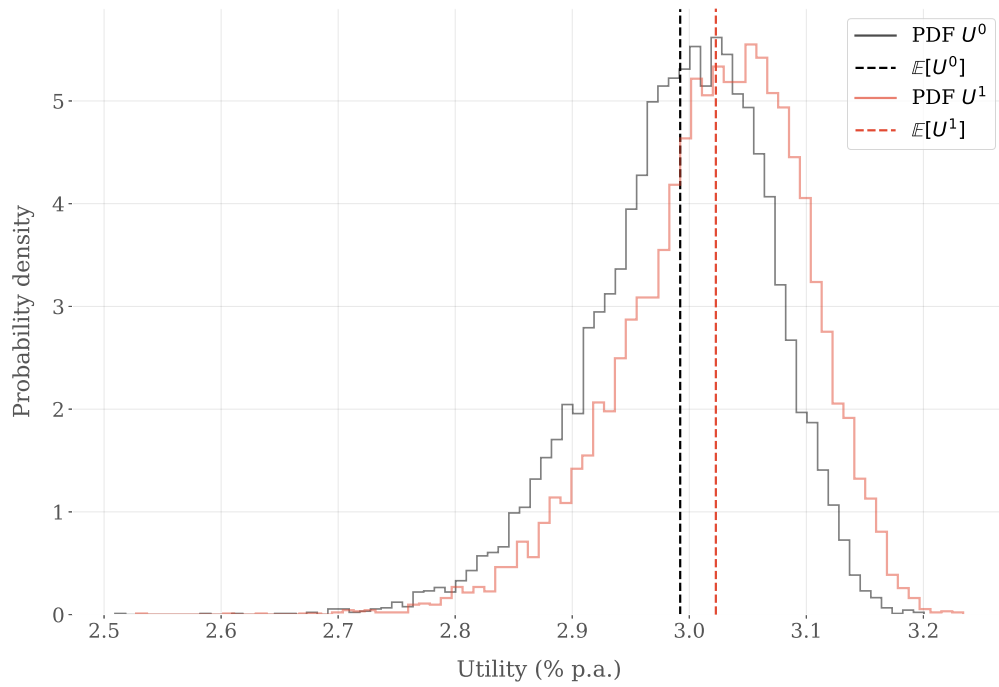
FIGURE 3. The simulated probability density functions for U^0 and U^1 (Equation 4) together with expected values.
