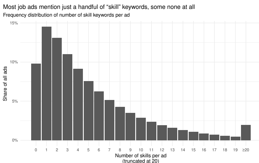
Figure 1: Number of skills per advertisement
