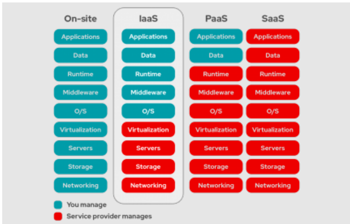
Figure 2 Service models of public cloud services
