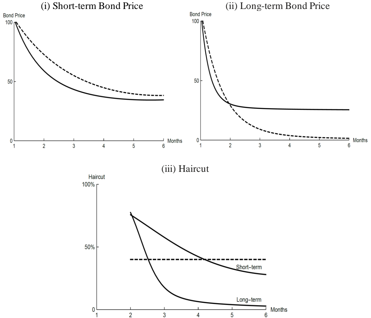
Figure 6: Uniform Exchange vs. Uniform Haircut: Bond Price Dynamics
