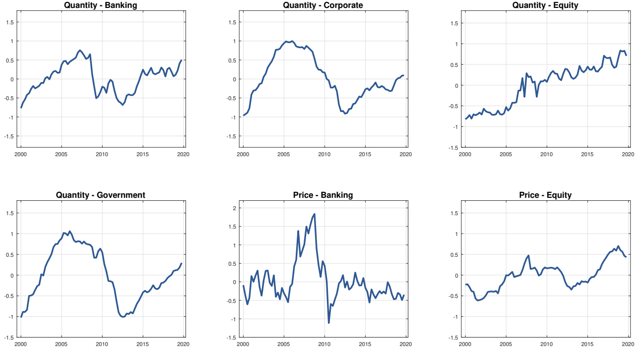
Figure 2: Auxiliary dataset.
