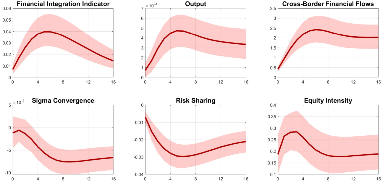
Figure 5: Impulse Response Functions - True Integration shock
