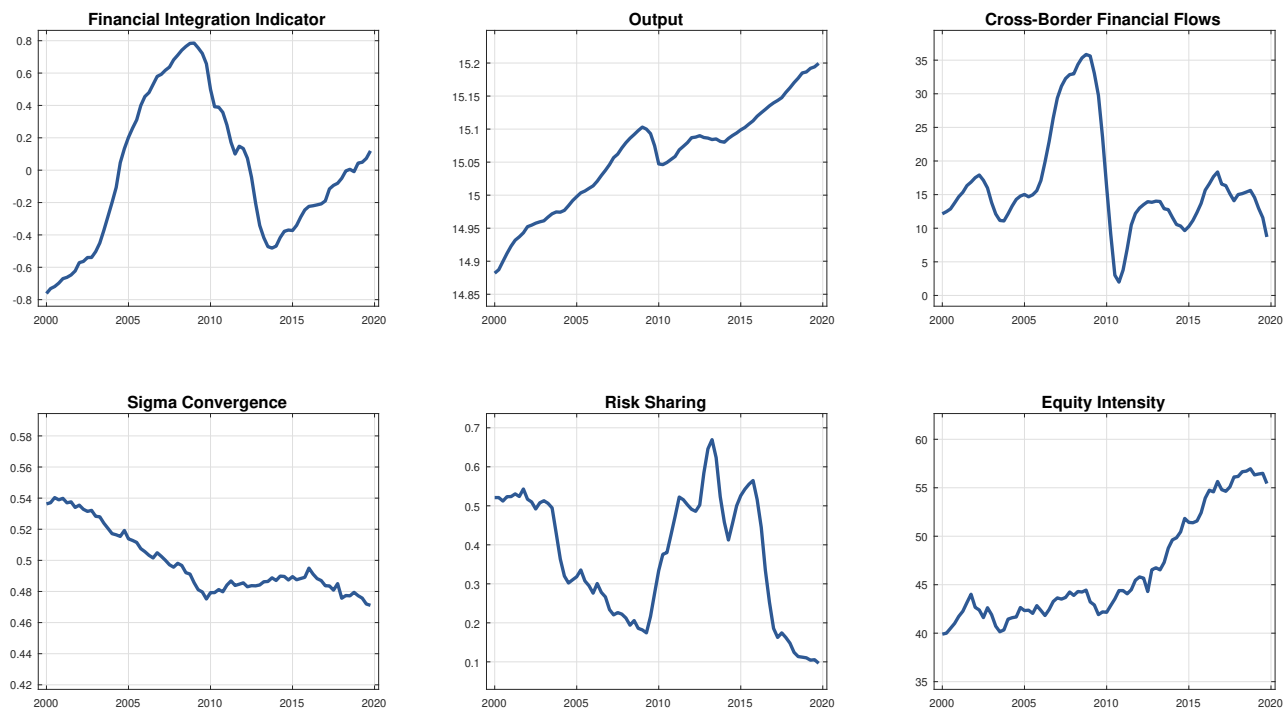
Figure 1: Main dataset.
