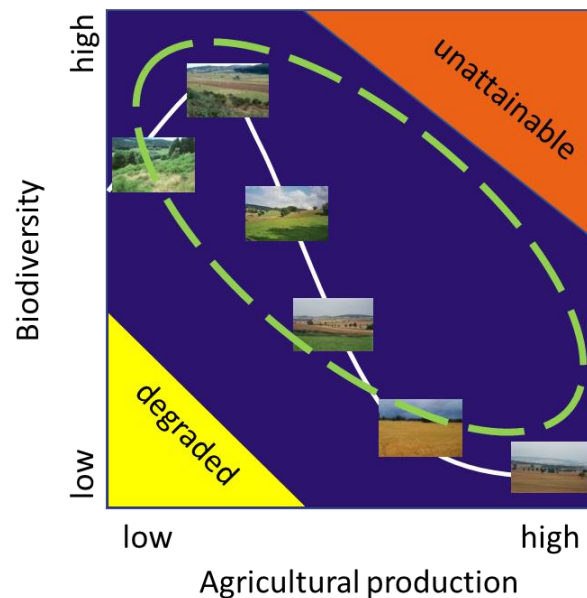
Figure 4: Schematic model of the relationship between biodiversity and agricultural production.
