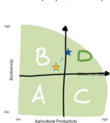
Scenario B (Graph Quadrants)
