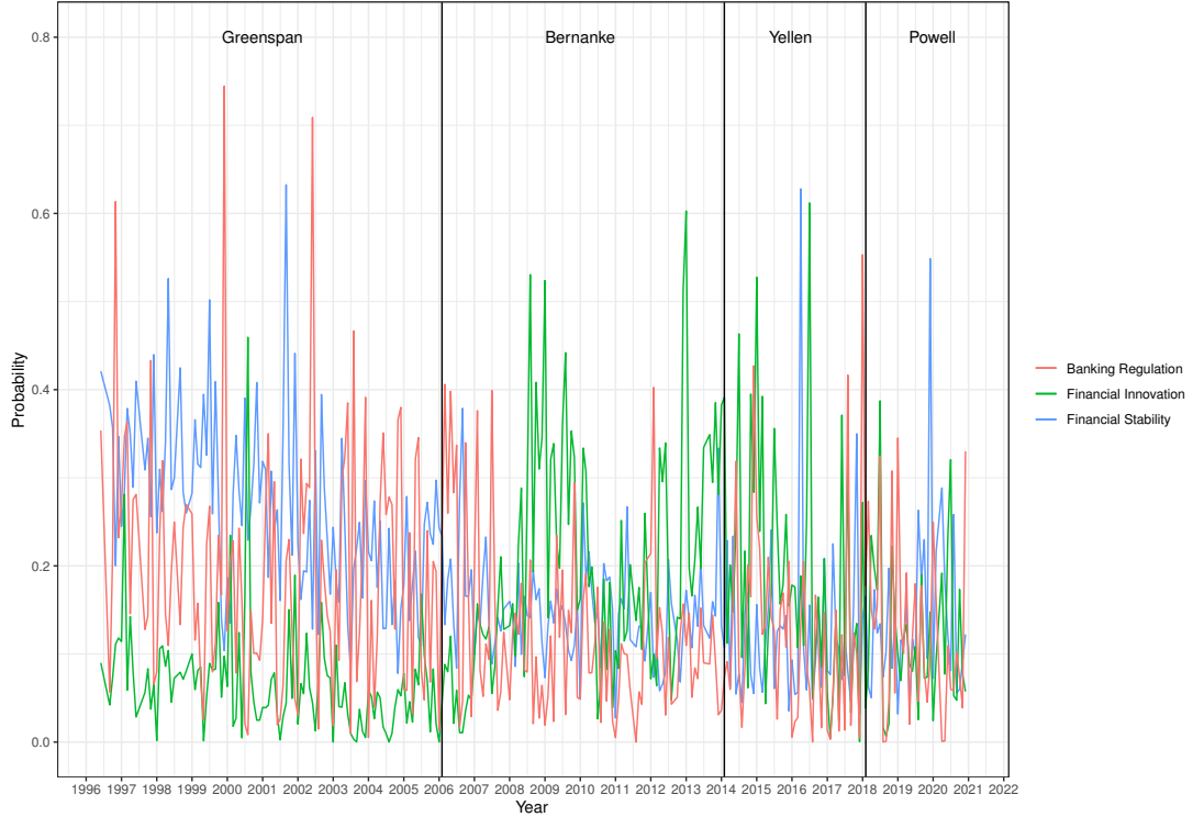
Figure 5: Evolution of non-keyword topic scores (monthly averaged) in the FED speeches.
