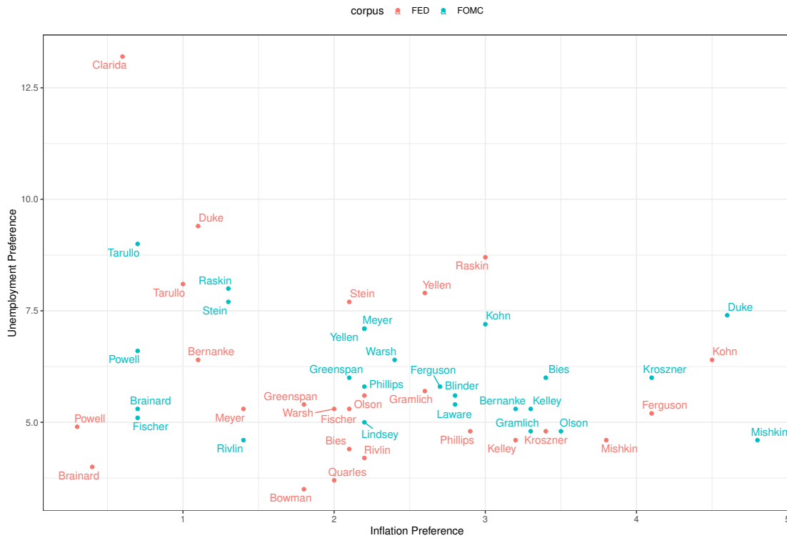
Figure 6: Biplot of estimated inflation and unemployment individual preferences.
