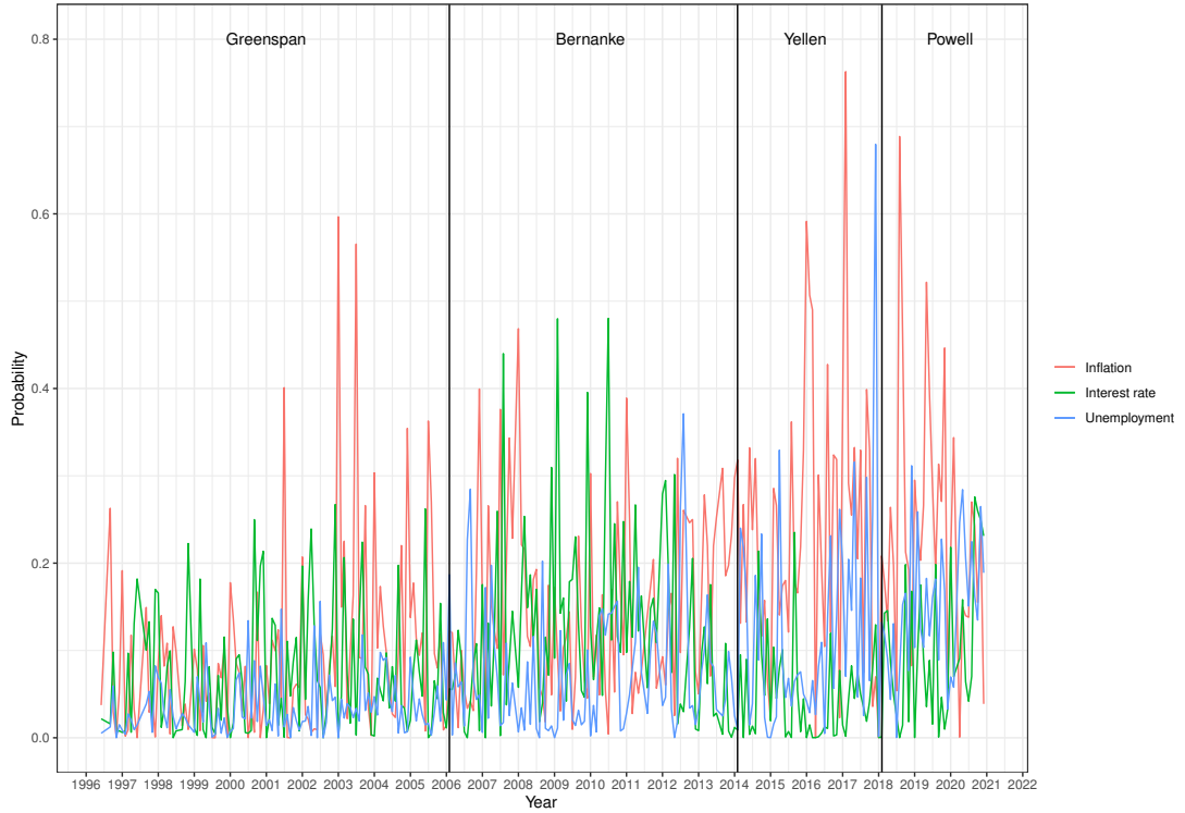
Figure 4: Evolution of keyword topic scores (monthly averaged) in the FED speeches.
