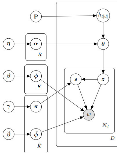
Figure 2: Graphical Model of the dynamic KeyATM (Eshima et al., 2020).
