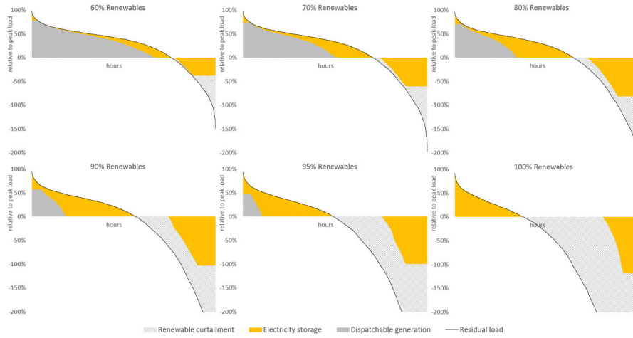
Figure SI.9: Residual load and electricity storage use in a setting with one dispatchable generation technology (hard coal) and one storage technology (pumped hydro storage), wind/solar PV capacity shares 25/75%.
