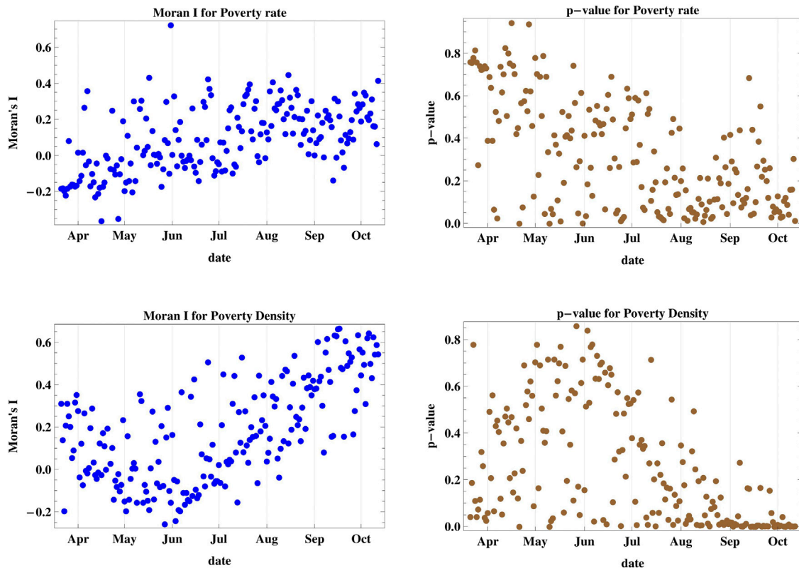
FIGURE 4 | Moran's I index and its corresponding p -value for cases V and VI accounting for regional poverty rate and poverty density. The poverty rate is not a decisive factor for spatial spread but when we consider the poverty density, we obtain spatial clustering starting on the end of August.
