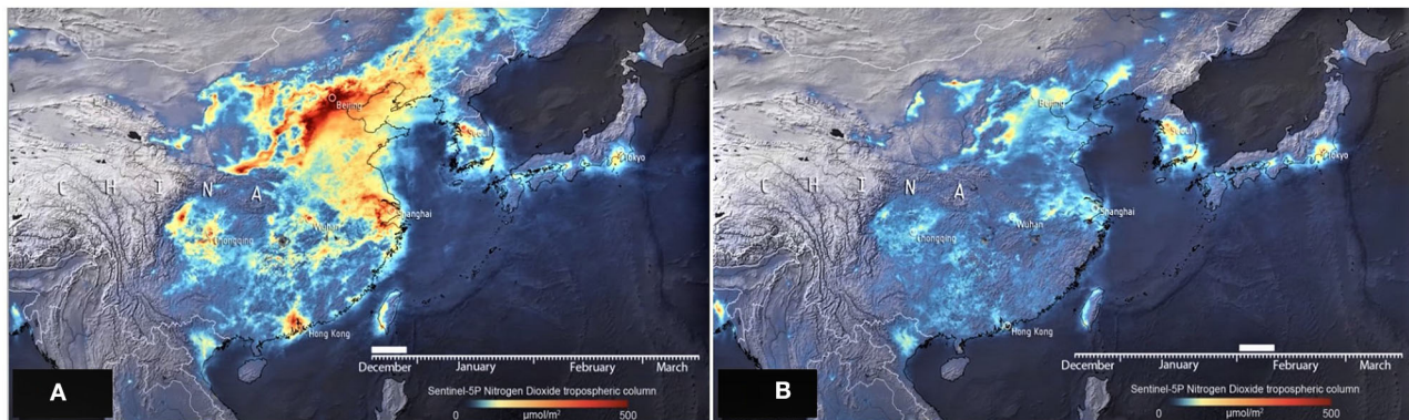
FIGURE 2 | \text{NO}_2 drops down in the coronavirus epicenter Wuhan, Hubei Province-China. (A) In December 2019, (B) February 2020 (4).
