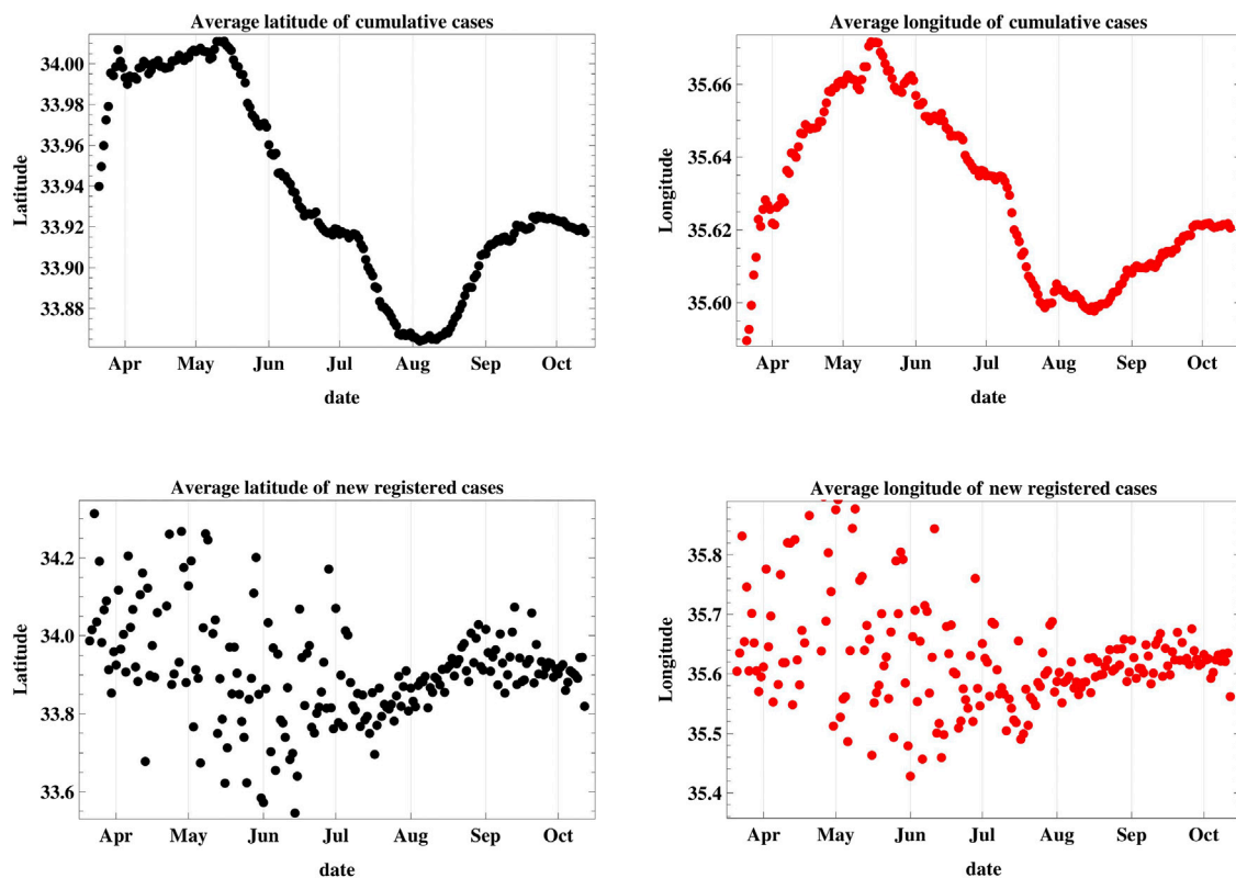
FIGURE 5 | This figure is a plot of the latitude and longitude of the weighted geographic center of COVID-19 infections in Lebanon. The upper graphs represent the temporal progression of the cumulative number of infections while the lower graphs represent that of the new daily cases.
