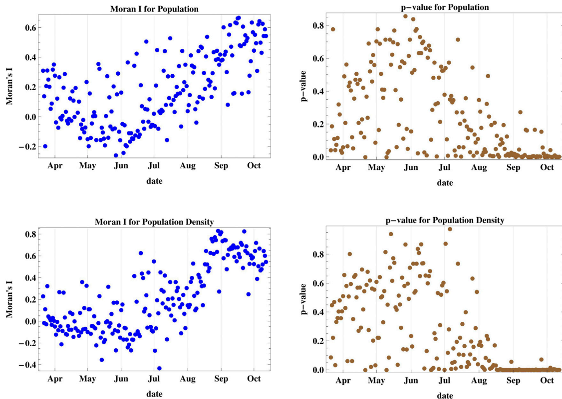
FIGURE 3 | Moran's I index and its corresponding p -value for cases III and IV accounting for population and population density of different districts. The daily spread was not clustered with respect to district population and density until late August 2020, where it started achieving strong spatial clustering between districts of adjacent population ranks.
