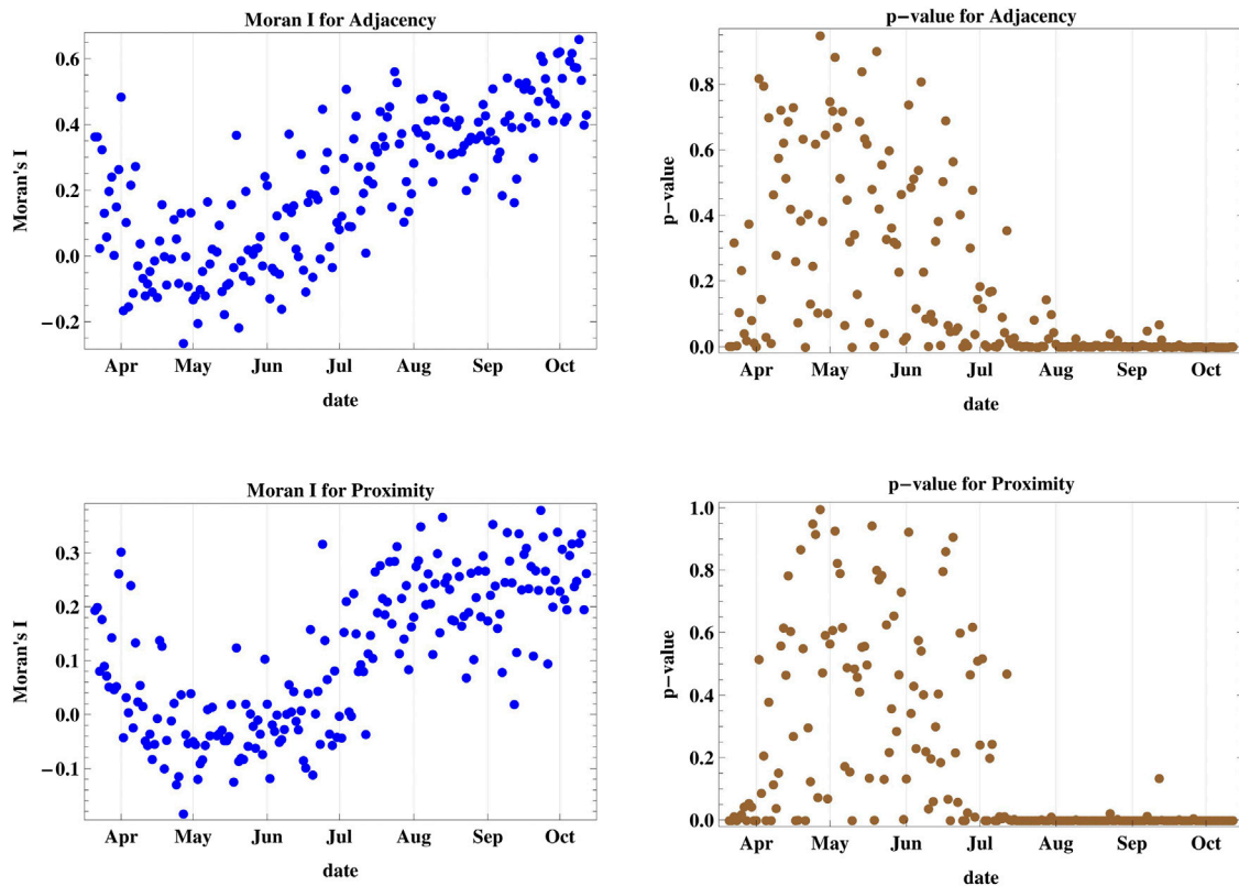
FIGURE 2 | The figure shows Moran's I index and its corresponding p -value for cases I and II accounting for adjacency and proximity of new infections registered in Lebanese districts. Since July, there is a strong clustering of daily infections in regions sharing common borders and among nearer regions.
