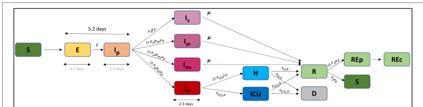
FIGURE 1 | Compartmental model. S, susceptible; E, exposed; Ip, infectious in the prodromic phase; Ia, asymptomatic infectious; Ips, paucisymptomatic infectious; Imms, symptomatic infectious with mild symptoms; Iss, symptomatic infectious with severe symptoms; ICU, severe case admitted to ICU; H, severe case admitted to the hospital but not in intensive care; REp, recovered without economic activity; REc, recovered with economic activity; D, deceased.
