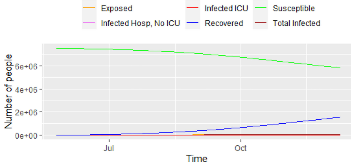
FIGURE 2 | Progress of the epidemic using model (1).
