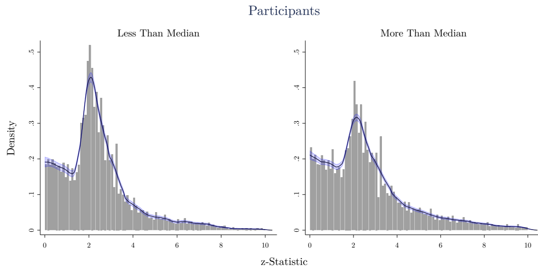
Figure 12: z-Statistics by Sample Size
