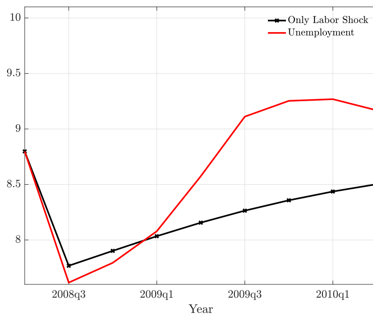
Figure 13: Counterfactuals for cyclical unemployment (black lines) and actual development (red line). Labor market performance shock only.
