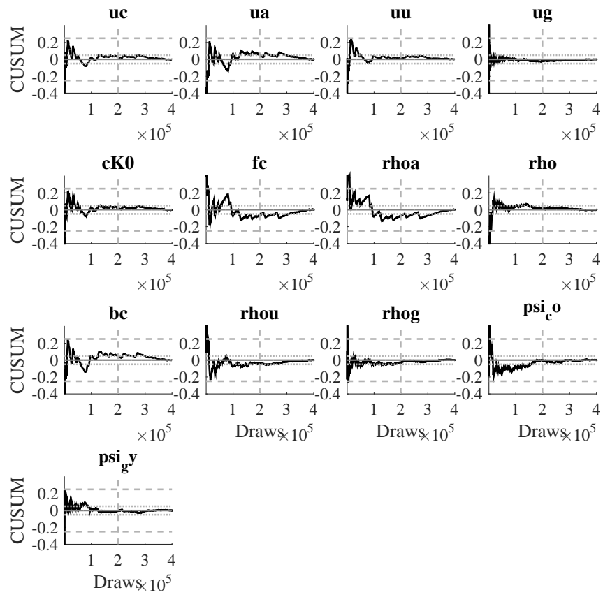
Figure 9: CUSUM statistics.
