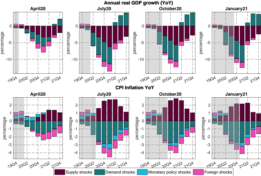
Figure 11: Shock Decompositions 2020-2021
