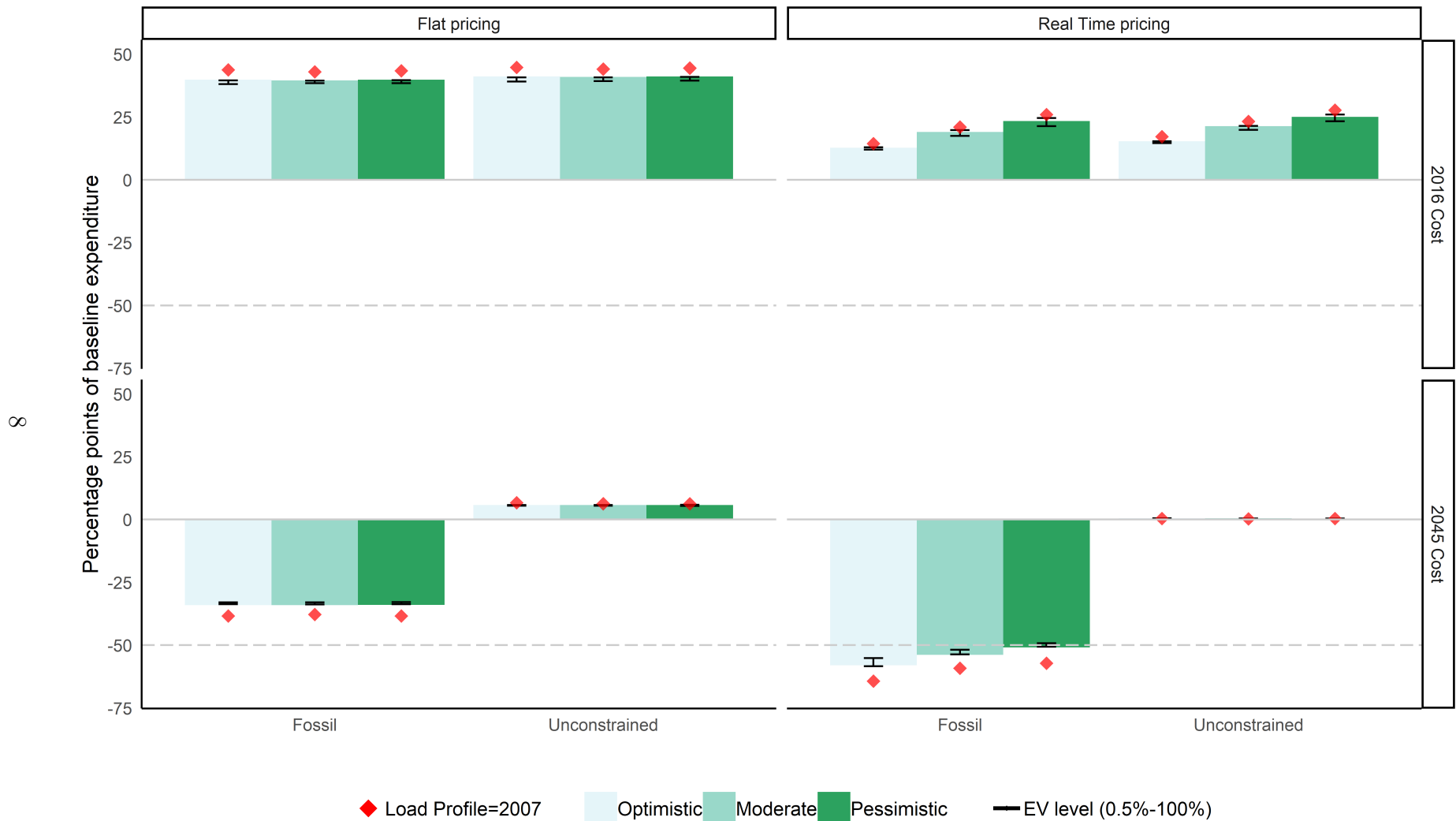
Figure S3: Cost of 100 percent renewable energy system relative to fossil and unconstrained systems under different cost and demand flexibility scenarios when the overall demand elasticity equals 0.5.
