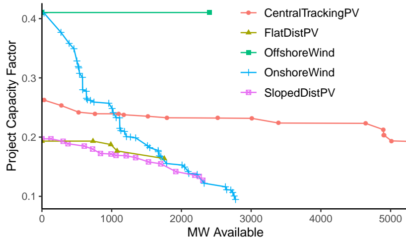
Figure 5: Average output and potential capacity of renewable energy sources on Oahu
