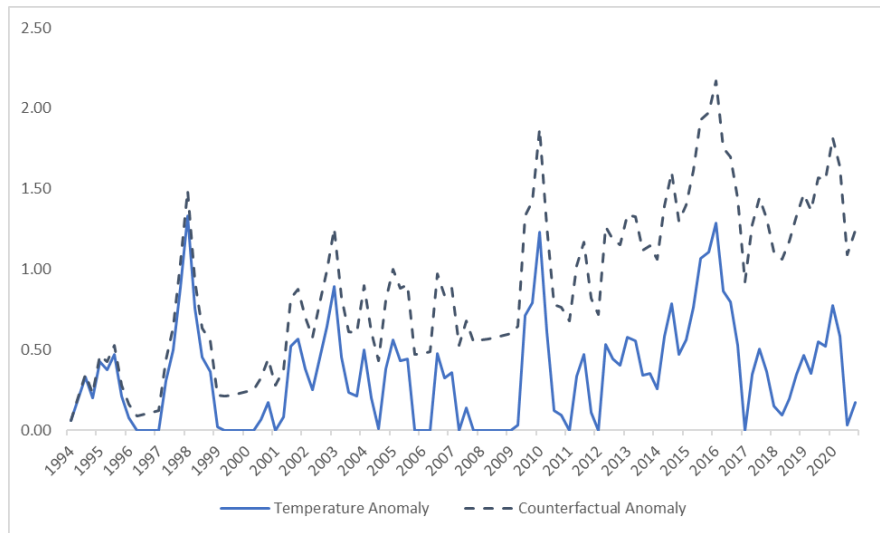
Figure 3: Temperature anomalies in Colombia and 1°C gradual warming
