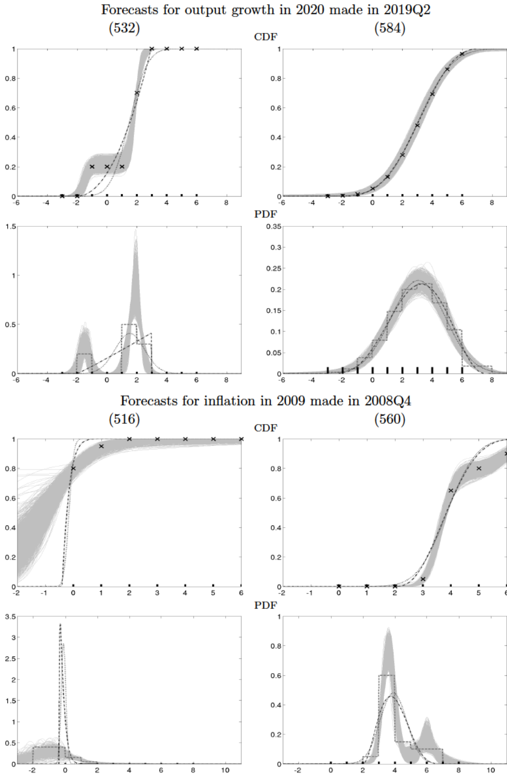
Figure 2: Inference using the Bayesian nonparametric approach: CDFs and PDFs for selected examples
