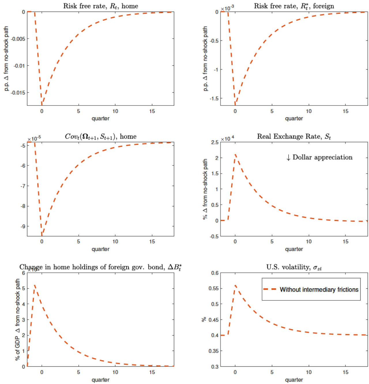
Figure 14: Impulse response functions of U.S. variables to a shock in the U.S. risk free rate
