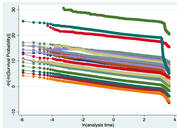
Figure C1: Estimated \log(-\log(\text{survival})) versus survival time for the 26 manufacturing classes
