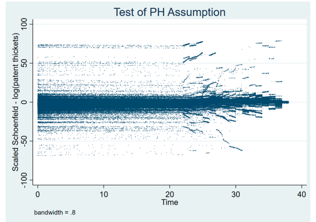
Figure C3: Schoenfeld residuals \log(\text{patent thickets})
