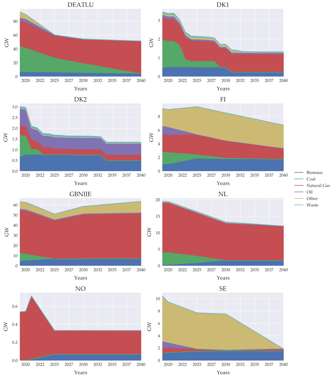
Figure A.4: Hourly average generation capacity for each country
