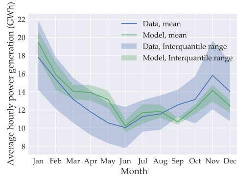
(b) Seasonality in aggregate generation
