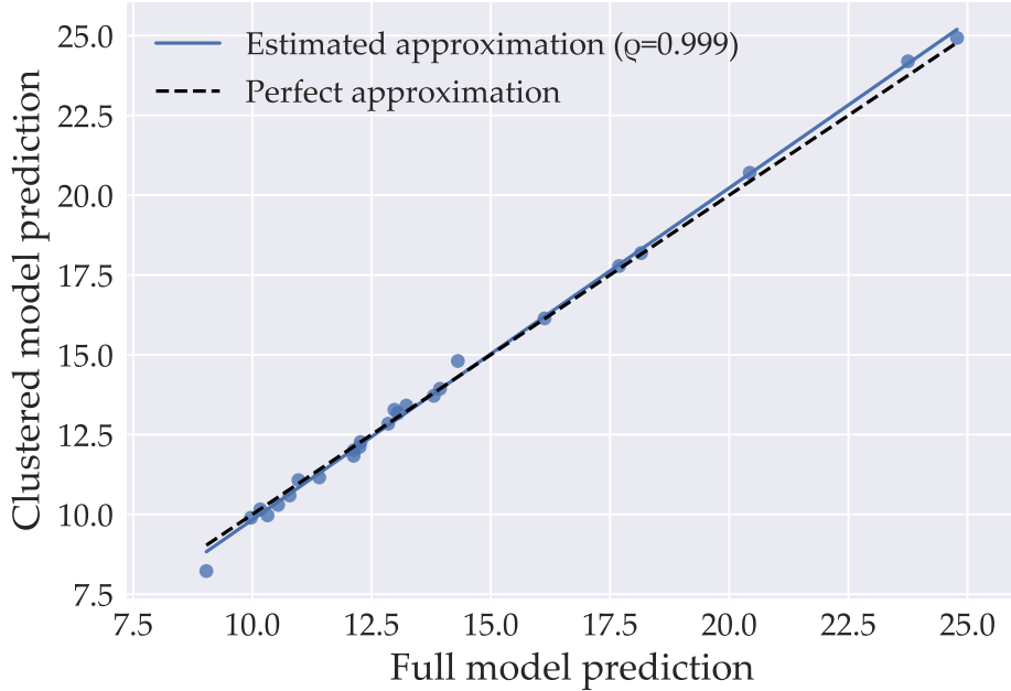
Figure 3.4: Optimal generation in full and clustered model, Norwegian hydro-model
