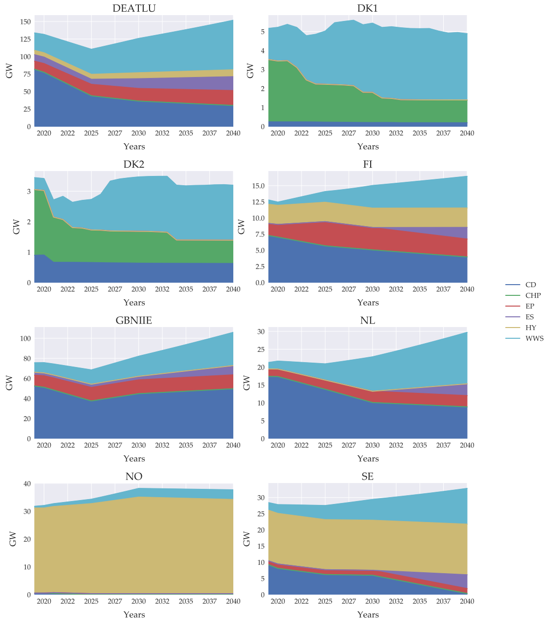
Figure A.3: Hourly average generation capacity for each country
