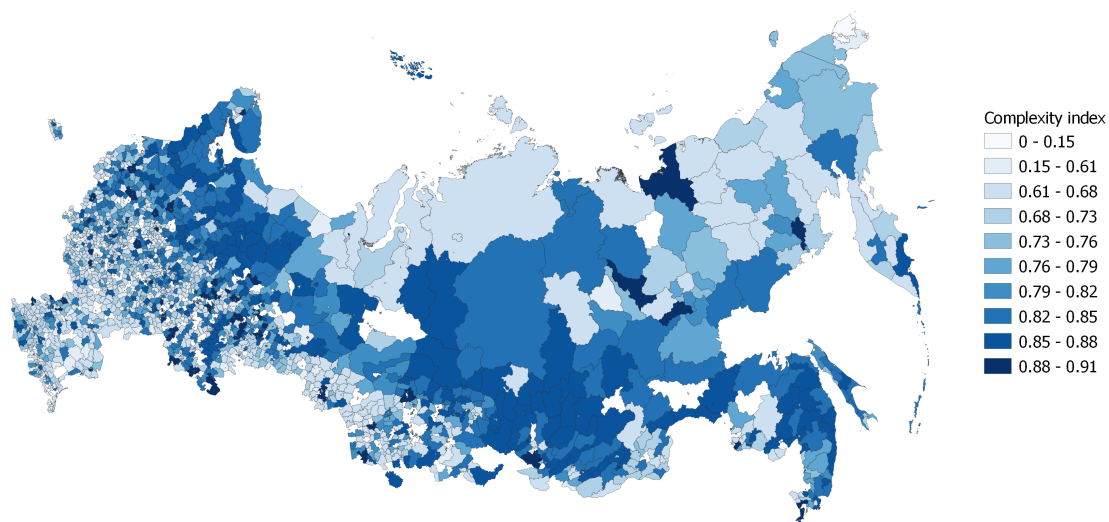
Figure 3: Complexity index
