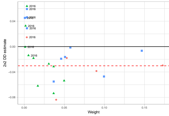
Figure A1: Goodman-Bacon (2021) decomposition: Low-track students, DV: Upper secondary school
