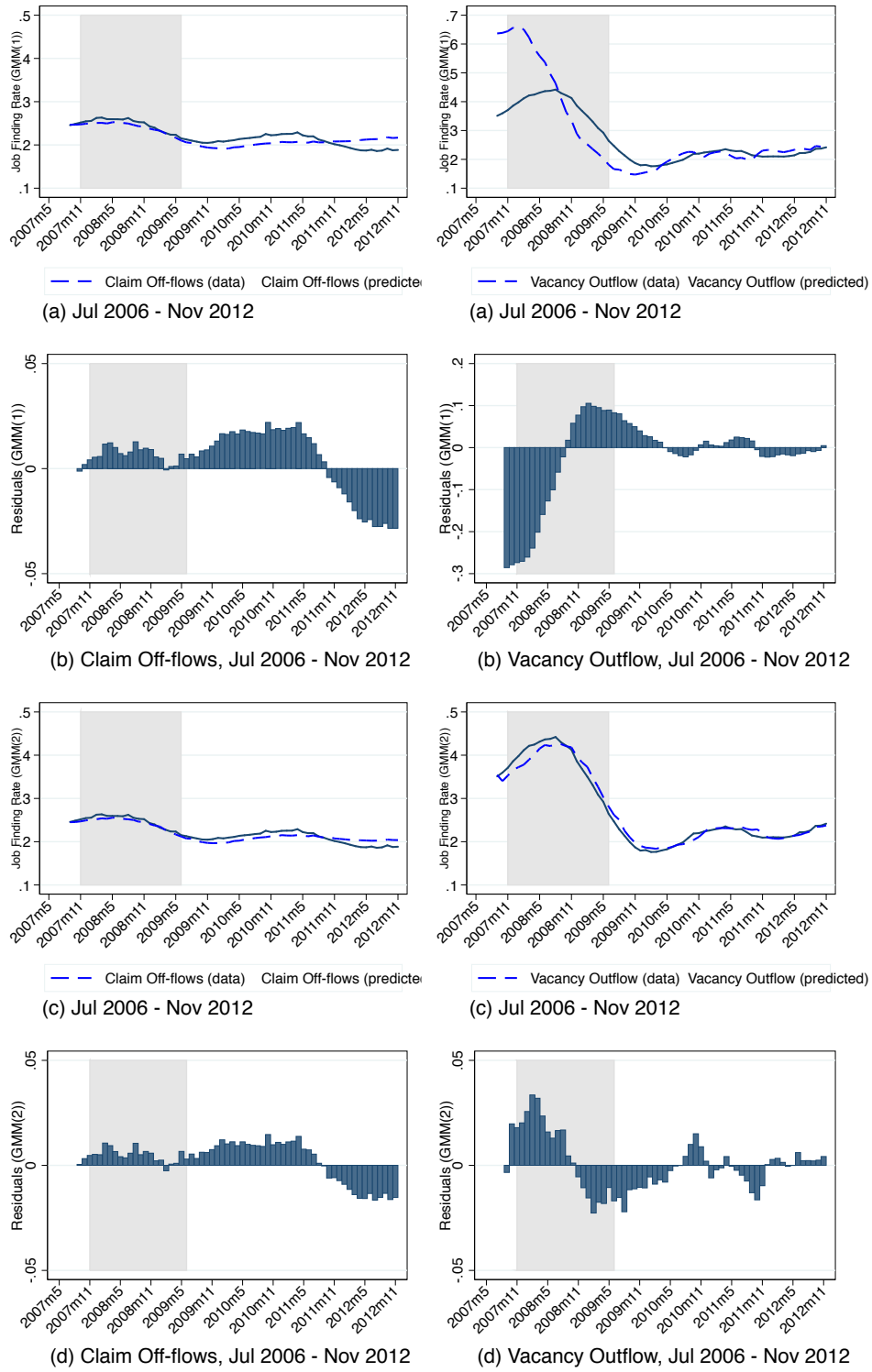
Figure 17: Job Finding Rate: The Aggregate Matching Function (Nomis-GMM)
