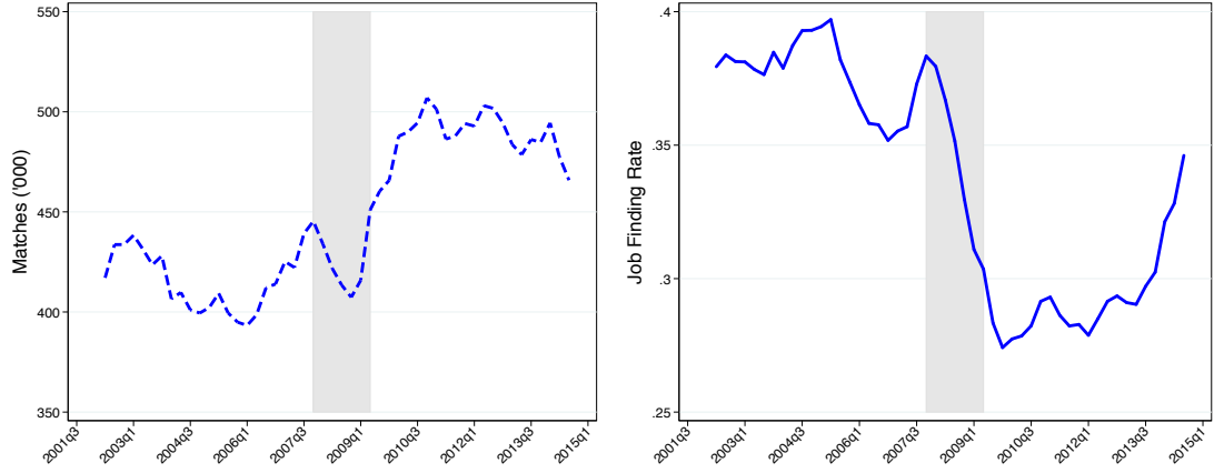
Figure 3: Matches and Job Finding Rate (LFS)
