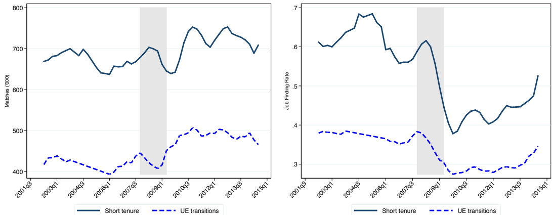
Figure 14: Matches and Job Finding Rate (LFS)
