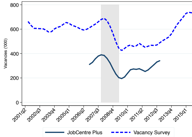
Figure 15: Aggregate Vacancies (Nomis and Vacancy Survey, Levels)
