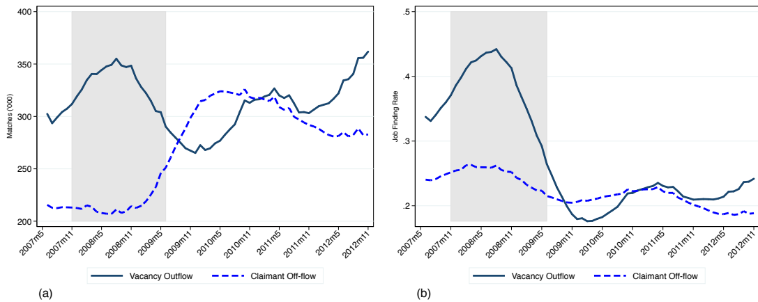
Figure 13: Matches and Job Finding Rate (Nomis)
