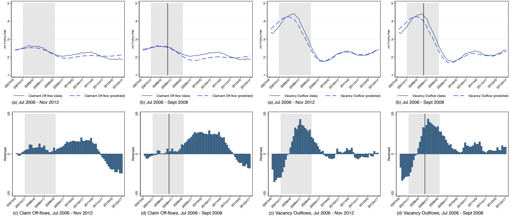
Figure 16: Job Finding Rate: The Aggregate Matching Function (Nomis-OLS)
