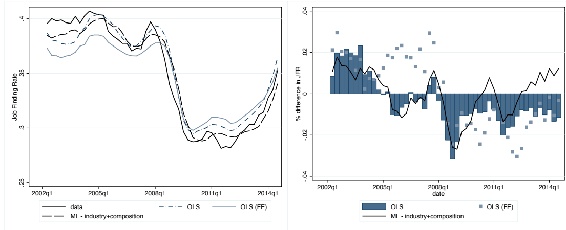
Figure 7: Job Finding Rates: ML estimation
