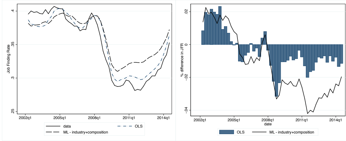
Figure 9: Job Finding Rates: ML estimation without unemployment duration Note: Predicted job finding rates and residuals from ML estimations on 2001Q3-2014Q3 period.
