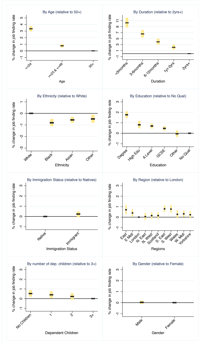
Figure 6: Job Search Efficiency: \beta
