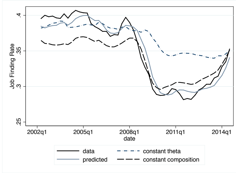
Figure 8: Counterfactual Job Finding Rates
