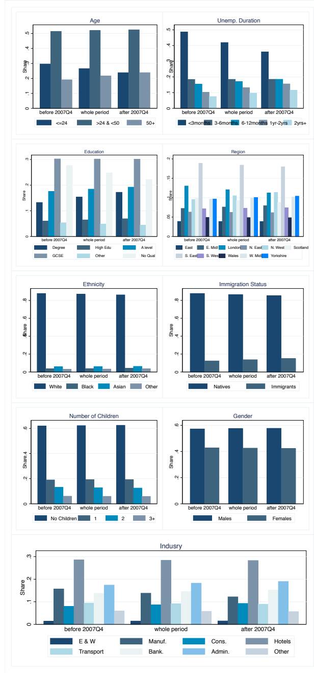
Figure 5: Worker composition: shares over time
