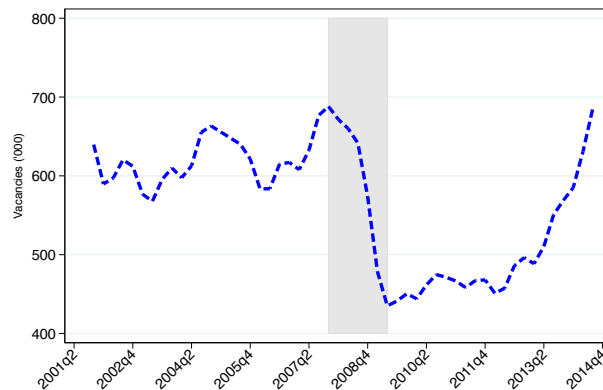
Figure 4: Aggregate Vacancies (Vacancy Survey, Levels)
