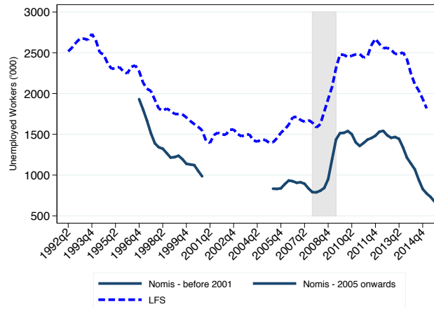
Figure 11: Aggregate Unemployment (Nomis and LFS, Levels)
