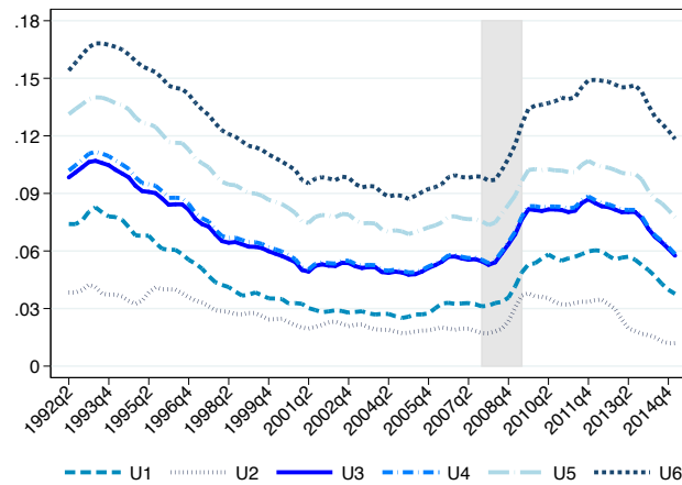
Figure 12: Alternative Measures of Unemployment
