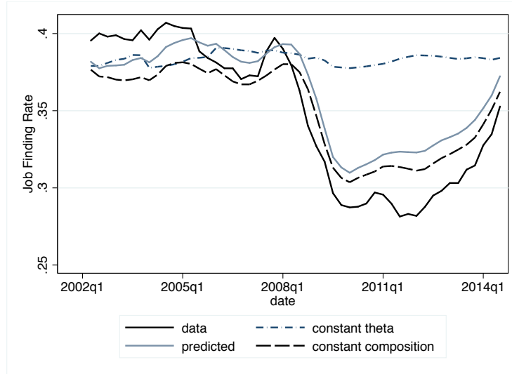
Figure 10: Counterfactual Job Finding Rates without unemployment duration Note: Predicted and counterfactual job finding rates from ML estimation on 2007Q3 - 2014Q3 period.
