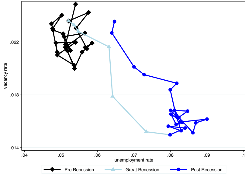
Figure 1: The Beveridge Curve
