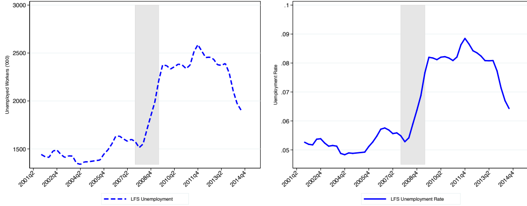
Figure 2: Aggregate Unemployment (LFS, Levels)
