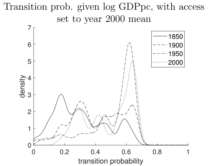
Figure 32: Demographic contagion
