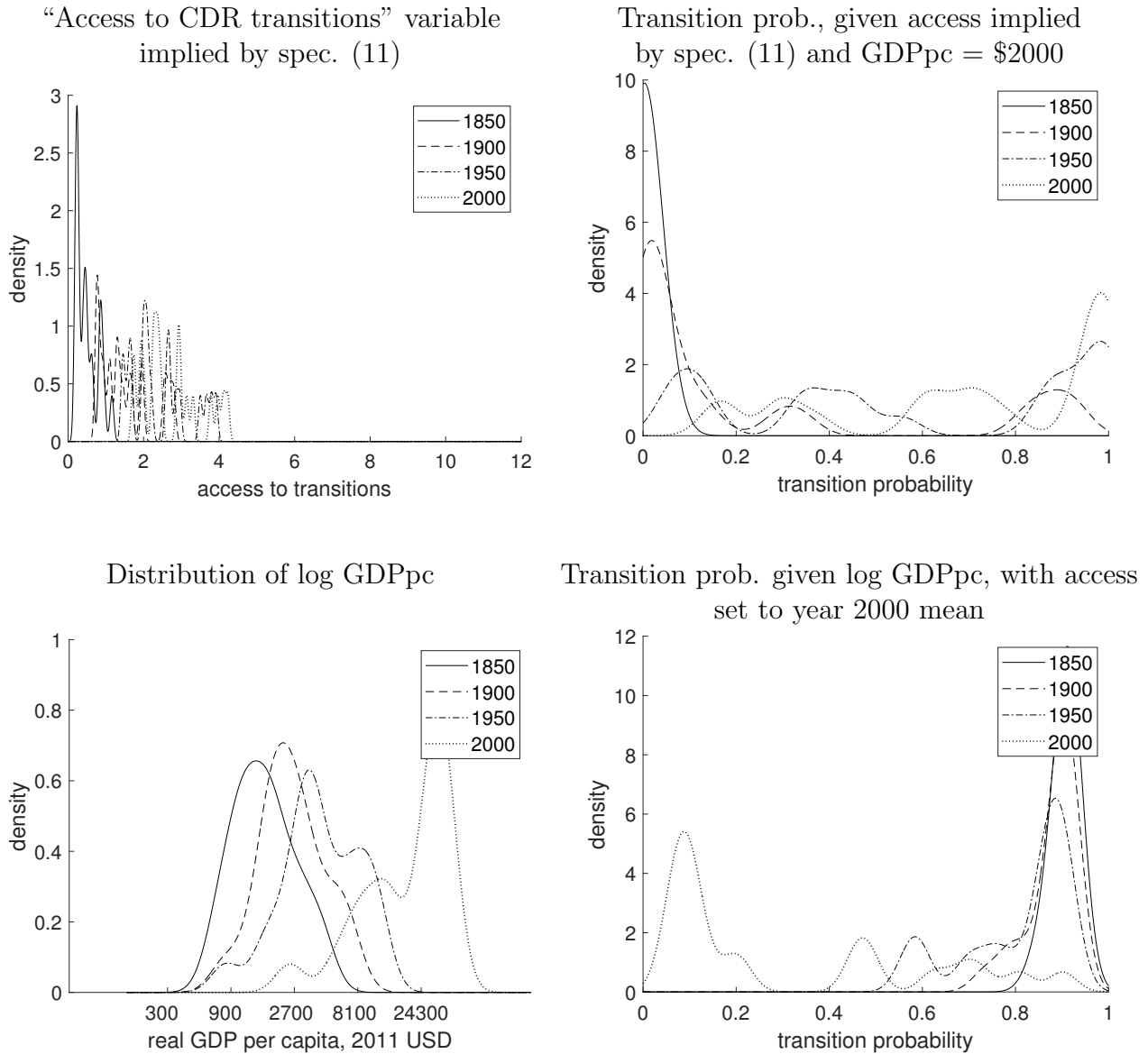
Figure 38: Demographic contagion
