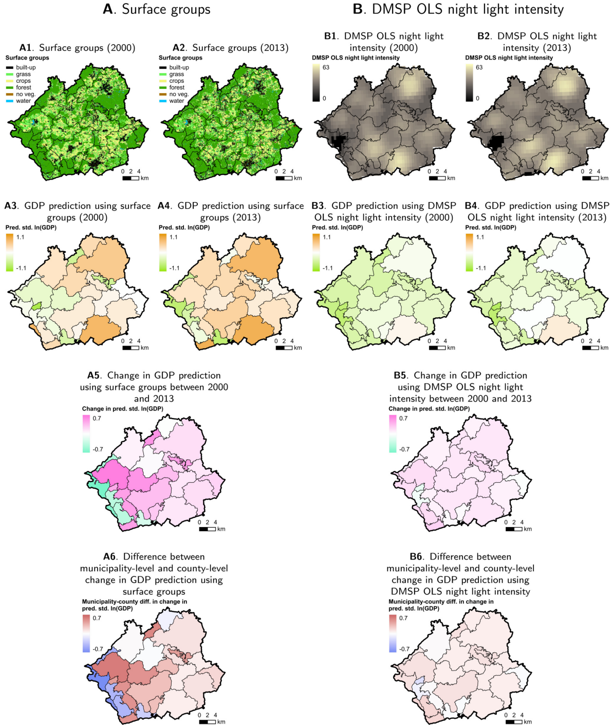
Fig. A9. Surface groups, DMSP OLS night light intensity, predictions of standardized \ln(\text{GDP}) , changes in predicted standardized \ln(\text{GDP}) , and municipality-county differences in the changes in predicted standardized \ln(\text{GDP}) . Maps show the county of Wunsiedel (situated in south-east Germany at the border to the Czech Republic).
