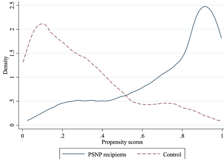
Figure A3. Propensity score common support
