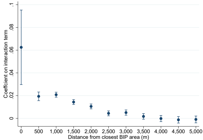
Figure 7: Spillover effects
