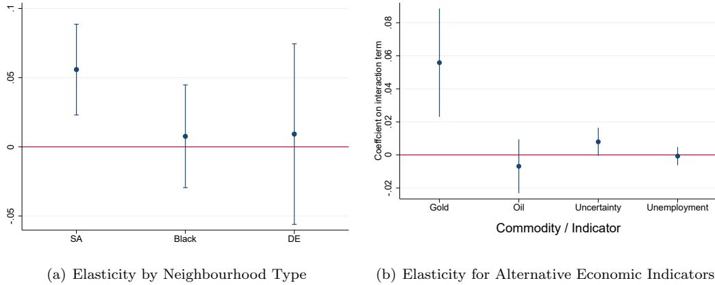
Figure 5: Falsification Exercise
