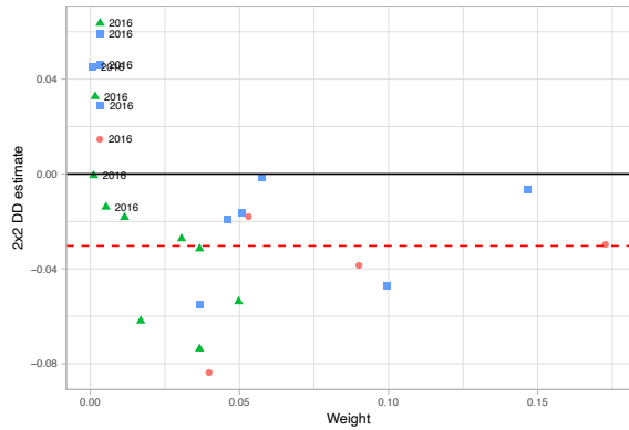
Figure A1: Goodman-Bacon (2021) decomposition: Low-track students, DV: Upper secondary school
